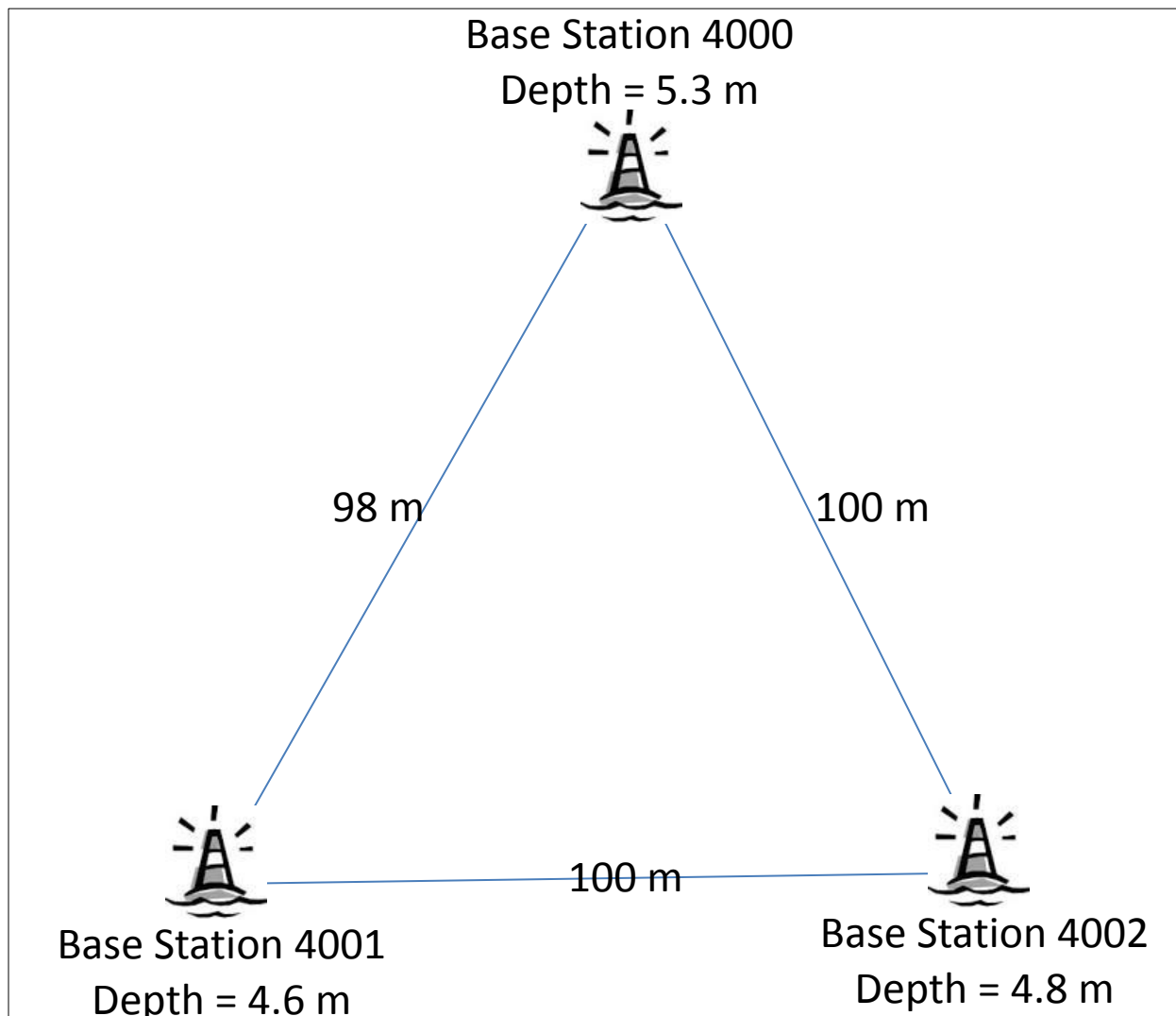
Figure 8: Deployment #2 layout
