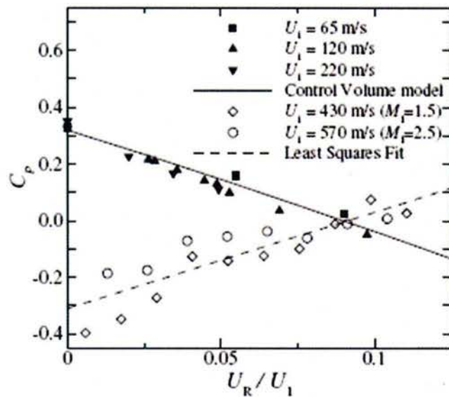
Fig. 4. Measured overall pressure coefficient vs. mass-injection ratio and chemical heat release.
