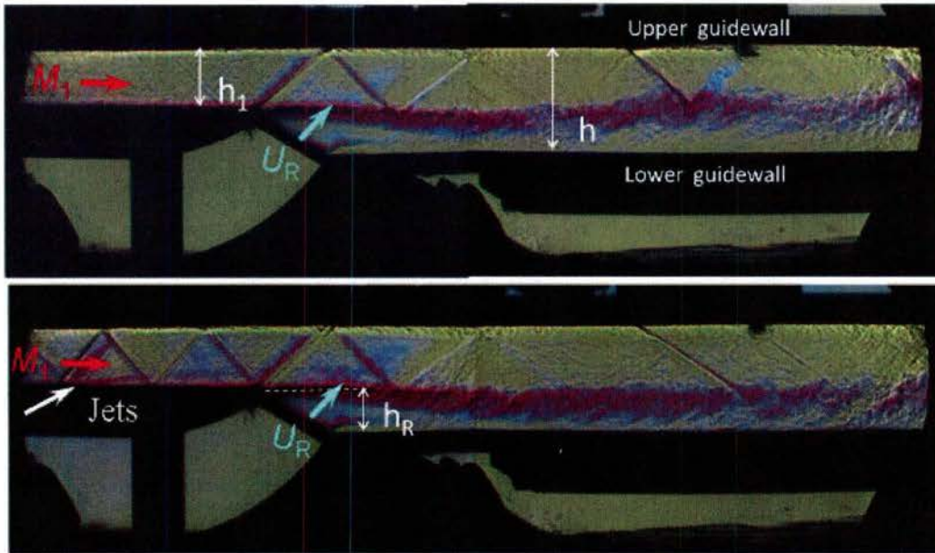
Fig. 7. Typical composite schlieren images obtained in the modified test section and nomenclature. Top: Ramp-injection only (without jet injection). Bottom: Combined ramp and inclined-jet injection. Both upper and lower streams are 100% [N 2 ].
