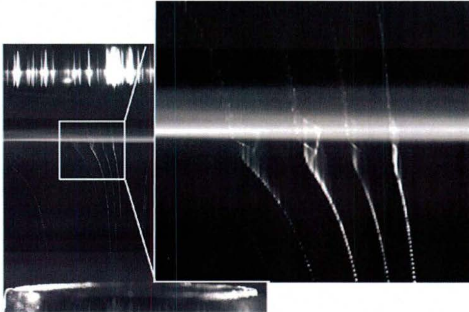
Fig. 19 Illustration of aero-optical effects. CH 4 -air flame, p = 6 atm, \Phi = 0.80 with N 2 used for both the co-flow and background gas. PTV trajectories are blurred by differences in refractive index between the flame and surrounding gases.
