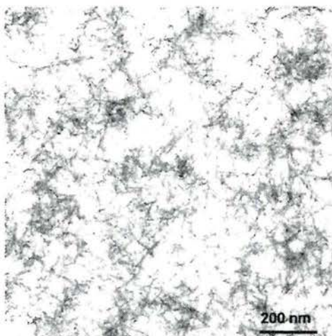
Figure 16. Above: Dispersion of nanorods in a P3Ht polymer film. Right, Controlled dispersion of hyperbranched CdSe in P3HT Polymer.
