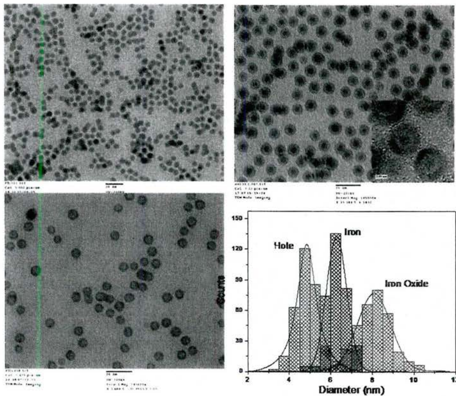
Figure 5. A wide range of materials can be made as hollow nanocrystals. This figure illustrates the formation of hollow gamma Iron Oxide (Fe 2 O 3 ). The initial Iron particles are exposed to Oxygen. The central void is a bit smaller than the original Iron, demonstrating the extent to which the oxygen penetrates the initial oxide shell. Many materials can be made hollow this way.
