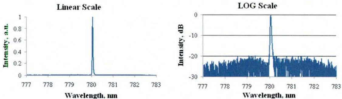
Fig. 25. Emission spectrum of a 7-module laser system operating at 200 W output power.
