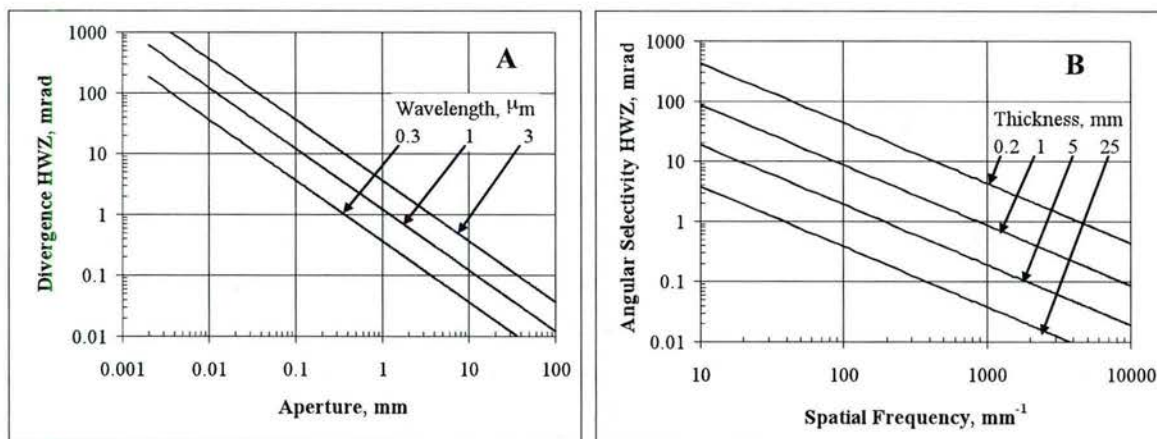
Fig. 1. Comparison of divergence of laser beams (A) and angular selectivity of Bragg gratings (B).
