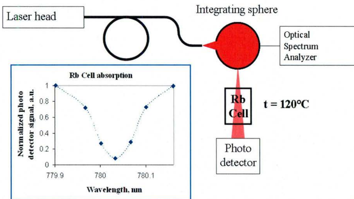
Fig. 26. Experimental setup to measure absorption of laser radiation in a Rb cell and dependence of cell transmittance on wavelength of a volume Bragg laser.
