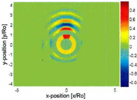
Fig. 5(a): GW field excited by a CLOVER sector ( 15 \mu s ) in an Al plate at 210 kHz-mm measured through laser vibrometry.
