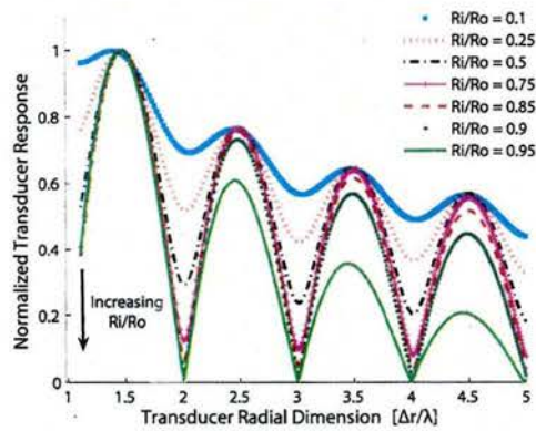
Fig. 2: CLoVER response as a function of transducer radial dimension: as the ratio of inner to outer radii ( R_i/R_o ) increases, the CLoVER sector approaches a symmetric rectangular geometry.
