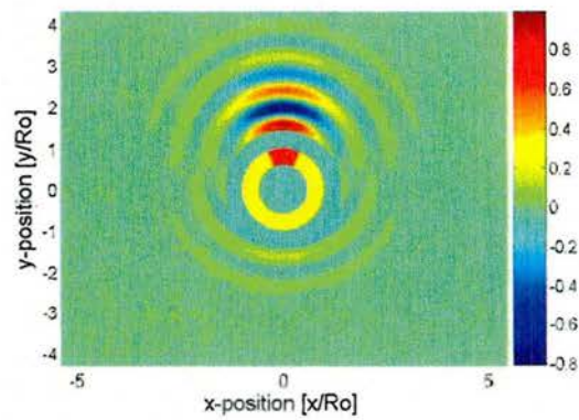
Fig. 5(b): GW field excited by a CLOVER sector ( 15 \mu s ) in an Al plate at 210 kHz-mm calculated using the theoretical model.
