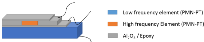
Fig. 2. Structure of a dual-frequency IVUS transducer.
