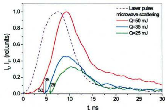
Figure 10: Measured Radar REMPI signal in air at pulse energies showing the delay in rise time associated with pulse energy. Arrows in Figure are predictions based on the laser pulse shape.
