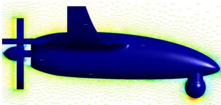
Figure 10. Flow Development around the Fuselage. Source: [17].
