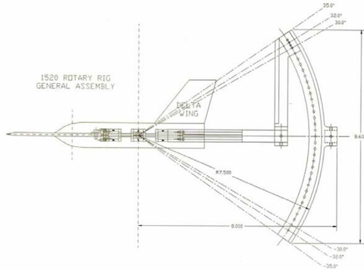
Figure 9. RHRC water tunnel rotary rig components. Source: [18].
