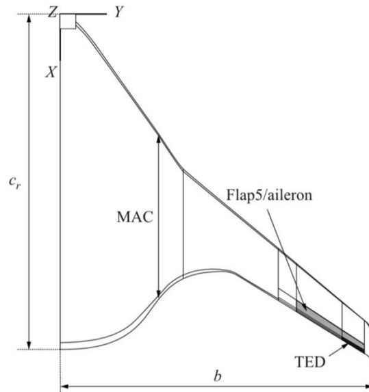
Figure 4. ACFA2020 with Flap5/aileron and TED. Source: [11].
