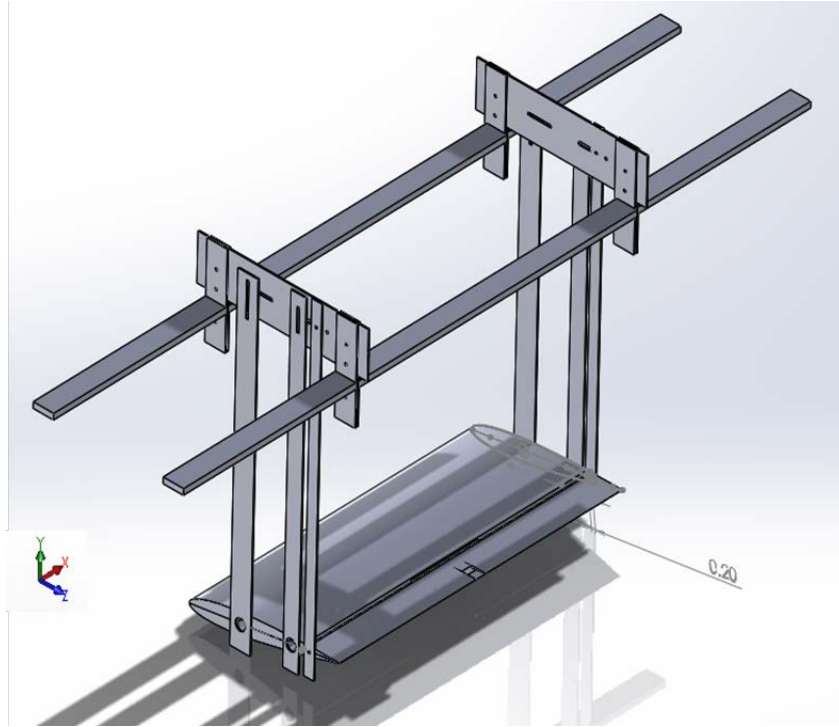
Figure 10. Aluminum airfoil holder array.
