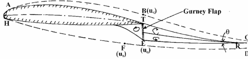
Figure 3. Flow pattern at the trailing edge with a Gurney flap. Source: [7].
