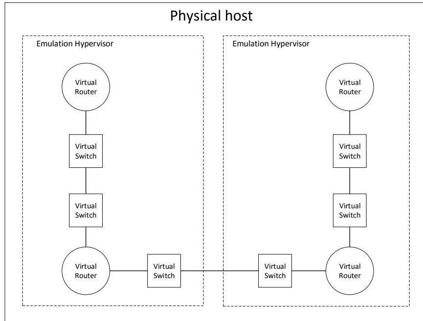
Figure 3.1: ERIK allows interconnections between hypervisors but does not support interconnections between physical hosts.
