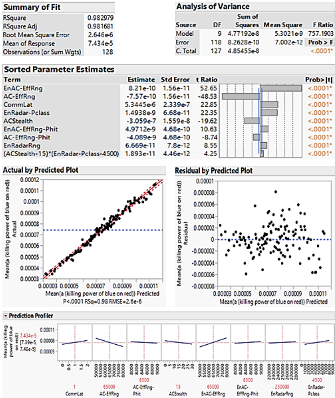
Figure 25. Regression Analysis of (a) Based on R5FF Data Library
