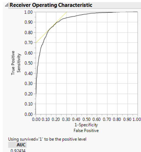
Figure 51. The ROC Curve for the First Nominal Logistic Regression for All Factors.
