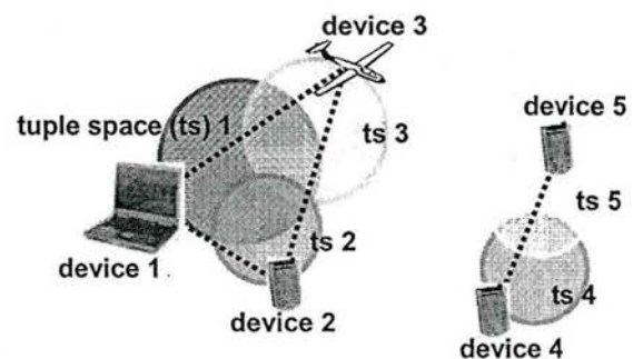
Figure 4: Dynamic coordination groups based on global virtual data structures. Devices 1, 2, and 3 form a group; devices 4 and 5 form a second group.
