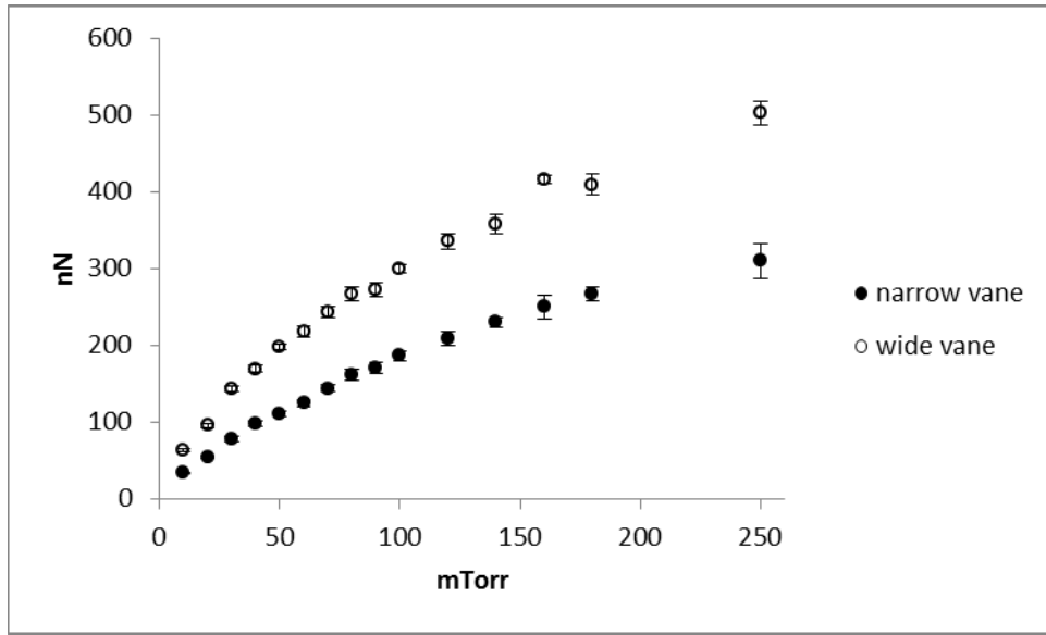
Figure 12. Drag Force at 10 rad/s (Simulation)
