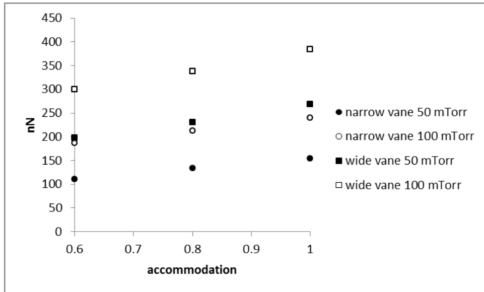
Figure 13. Drag Force with Varied Accommodation (Simulation)
