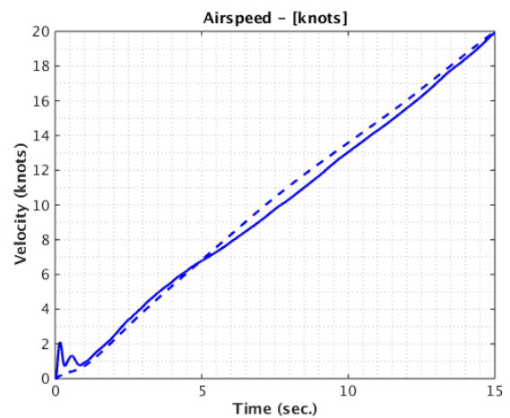
Figure 6. Variations in airspeed of the simulated helicopter accelerating IGE z=1R above ground.
