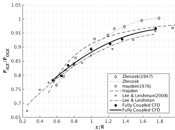
Figure 1 - Normalized main rotor power required for a helicopter hovering at different altitudes above ground.
