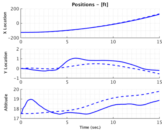
Figure 3. Variations in positions of the simulated helicopter accelerating IGE at z = 1R above ground.
