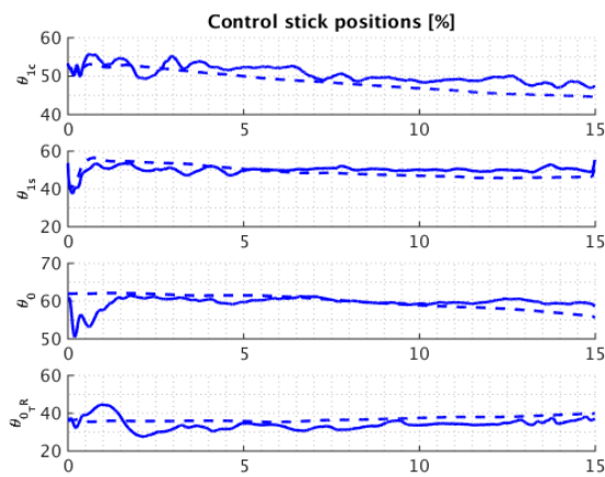
Figure 3. Variations in positions of the simulated helicopter accelerating IGE at z = 1R above ground.
