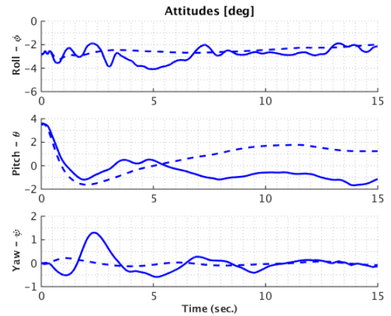
Figure 4. Variations in attitudes of the simulated helicopter accelerating IGE at z = 1R above ground.
