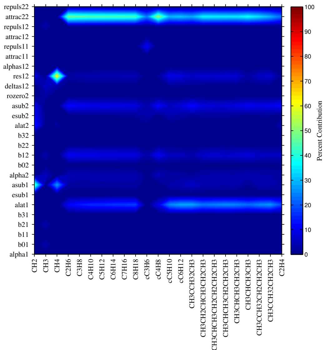
Fig. 8 Summary of ANOVA results for the H-C-H bond angles of all molecules examined. The percent contribution by each of the MEAM parameters was determined by dividing the sum of squares attributed to each parameter by the total sum of squares (e.g., see Table 4), which was repeated for each molecule. The mean bond angle for all H-C-H bond angles was used for those molecules with multiple H-C-H bond angles.
