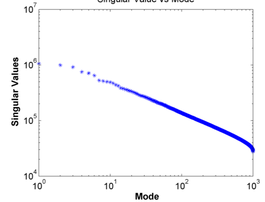
Singular Value vs Mode
