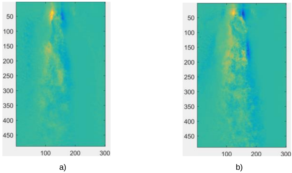
Figure 14 – The DMD spatial mode extracted from the high-speed shadowgraphy for a) 1920 Hz, and b) 3060 Hz. The alternating band is indicative of a in-plane flapping.
