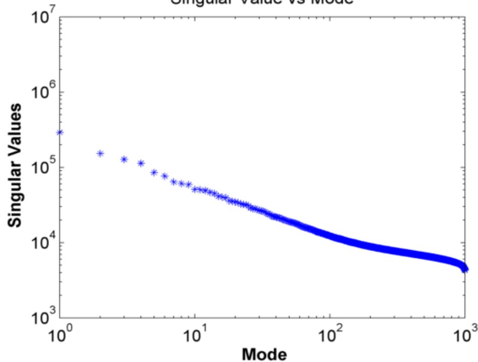
Singular Value vs Mode
