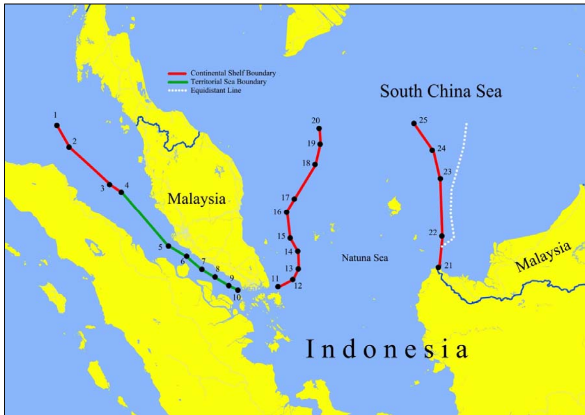
Figure 3. Indonesia and Malaysia Maritime Boundaries
