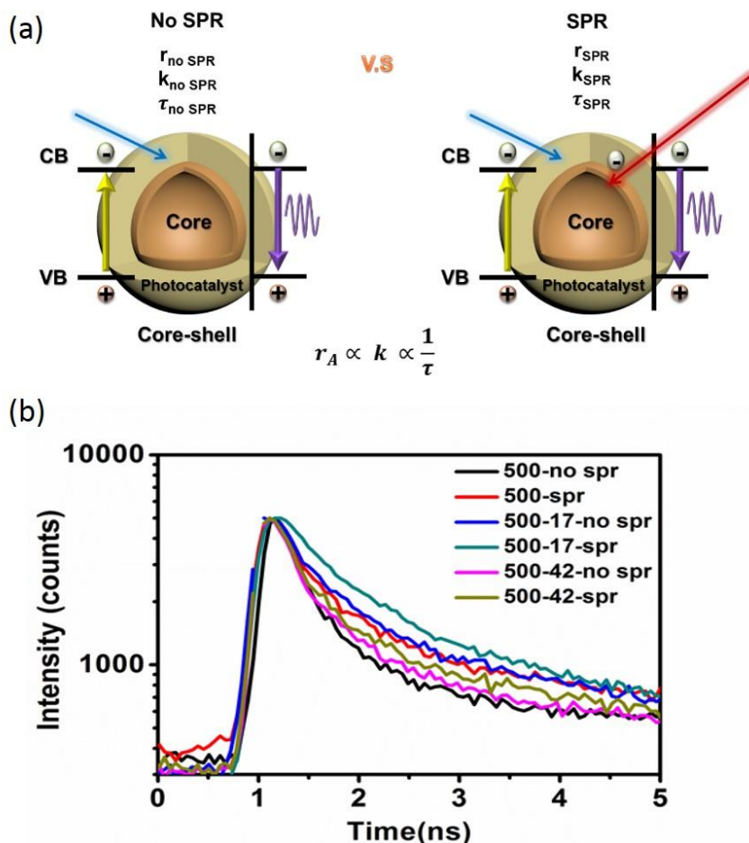
Figure 2. Time-resolved photoluminescence experiment (a) single pulse laser excitation (left) and single pulse laser excitation with continuous-wave light excitation (right). (b) PL intensity decay spectra.
