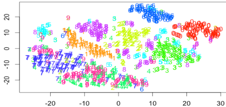
Figure 8. Rtsne 2D plot of MNIST data
