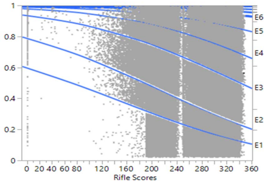
Figure 21. Pattern Analysis
