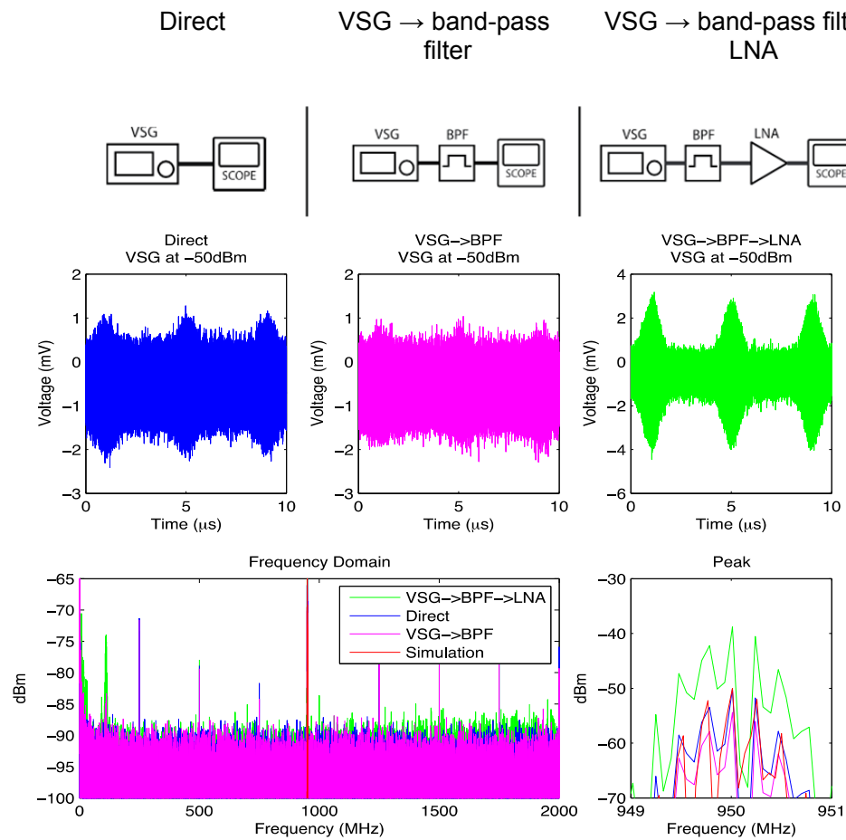
Figure 17. Experimental measurements taken with a VSG at -50 dBm comparing results taken directly through the band-pass filter, and through the band-pass filter, followed by an LNA.
