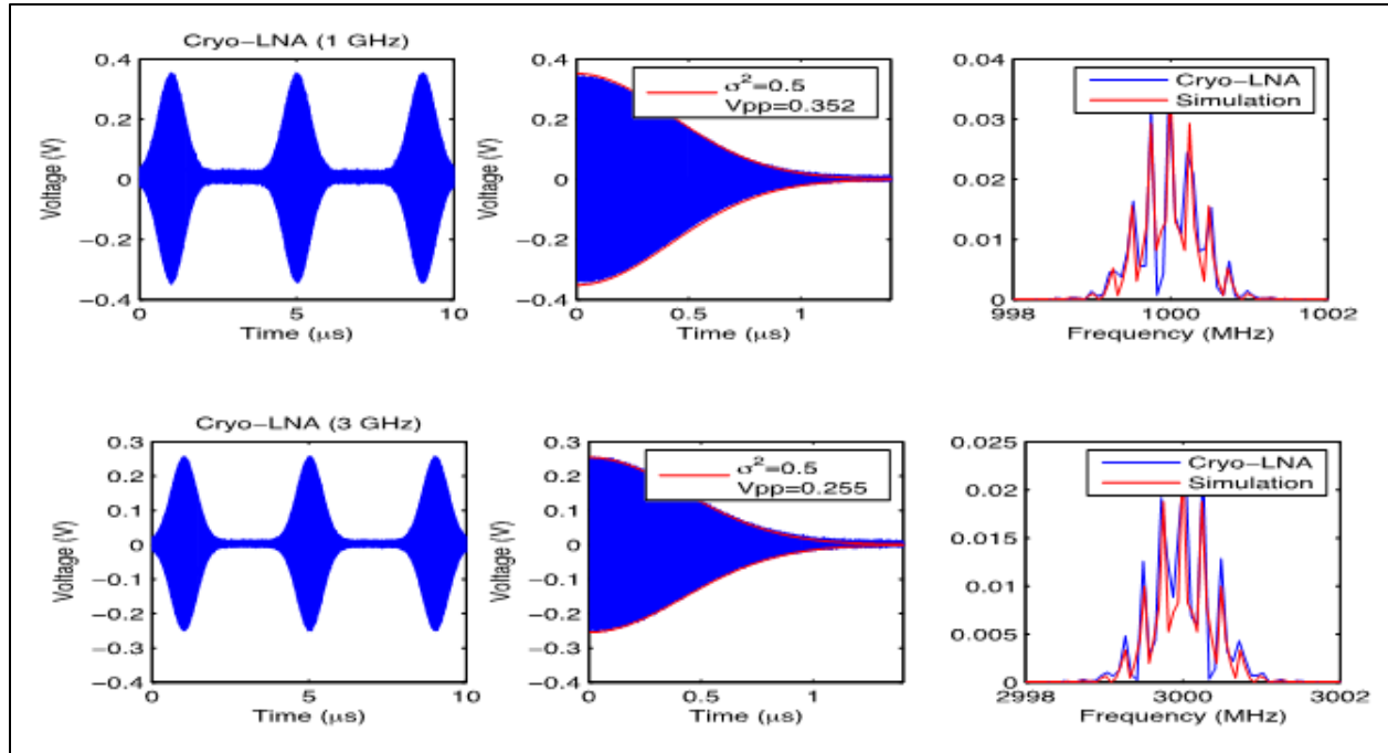
Figure 10. Measured pulses in time and frequency domain in comparison with an ideal Gaussian envelope pulse carrier of 1 GH.
