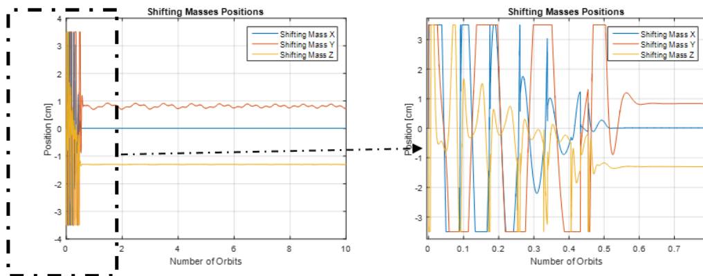
Figure 57. Shifting Masses Positions (Three Shifting Masses with Magnetorquer)
