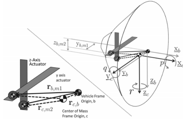
Figure 12. Proposed Method for Angle-of-Attack and Sideslip Angle Control
