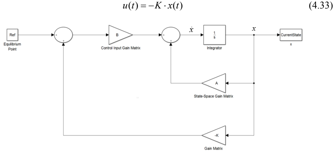
Figure 52. State Feedback Control Block Diagram
