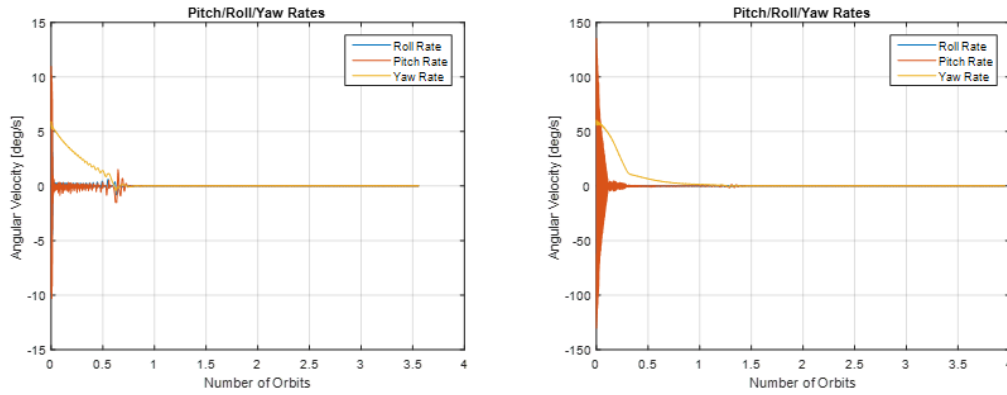
Figure 79. Initial Angular Rate Trials
