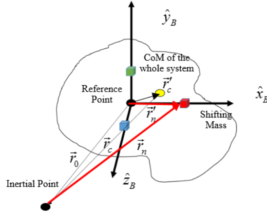
Figure 50. System Geometry
