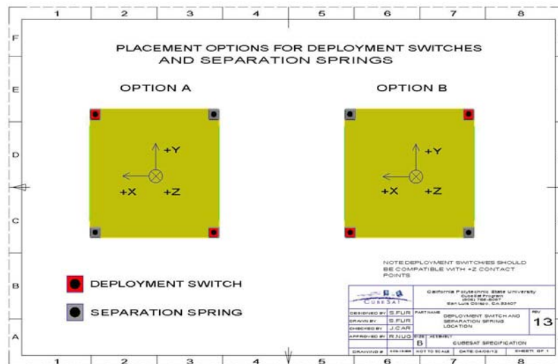
Figure 7: Deployment Switches and Separation Spring Locations
