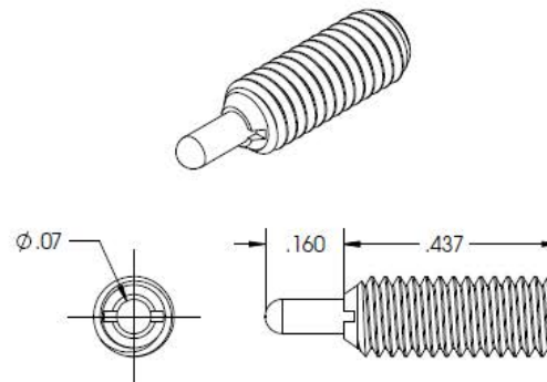
Figure 5: Custom Spec Spring Plunger (Separation Spring)
