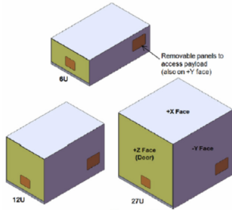
Figure 3. Canisterized Satellite Dispenser
