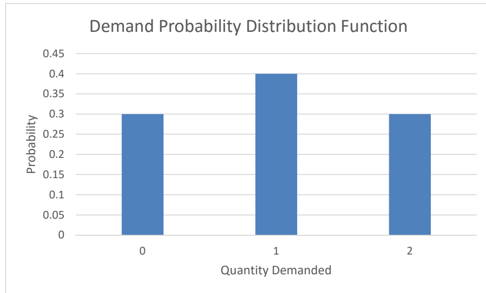
Figure 5. Resulting DPDF
