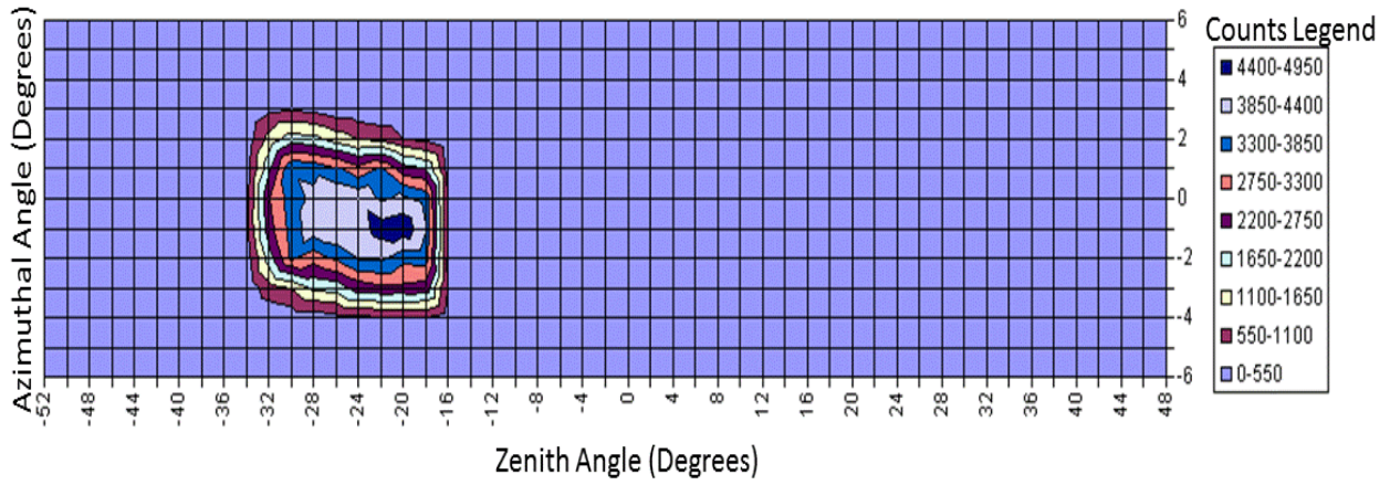
Figure 9. SSJ5 SN16 zone 5 angular response to 1350 eV electrons measured on 10/25/01
