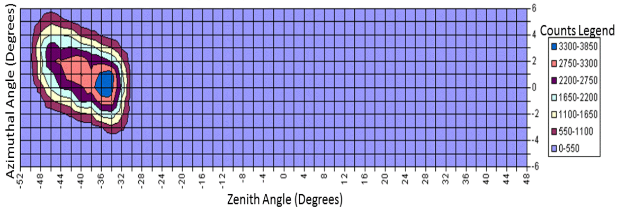
Figure 10. SSJ5 SN16 zone 1 angular response to 1350 eV electrons measured on 10/25/01
