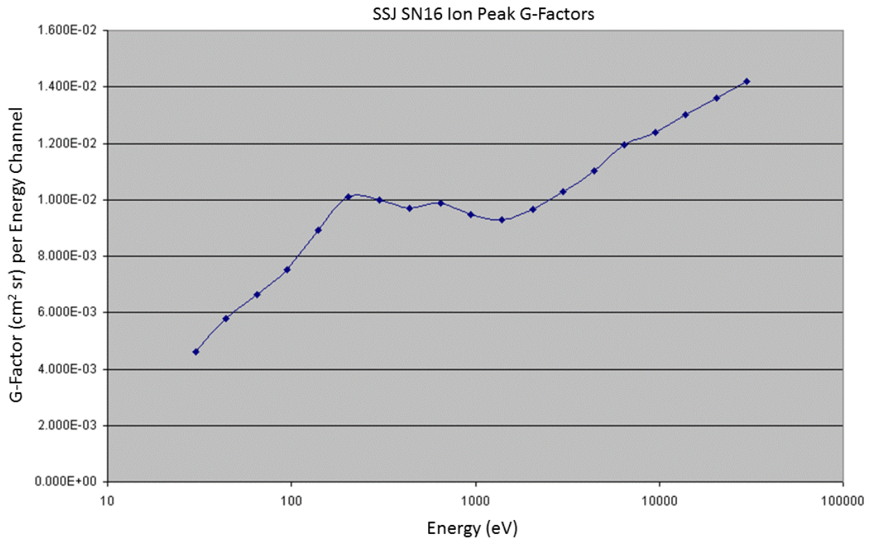
Figure 21. Mode A ion peak geometric factors from Table 4
