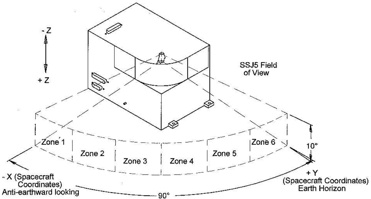
Figure 1. SSJ5 field of view and zones
