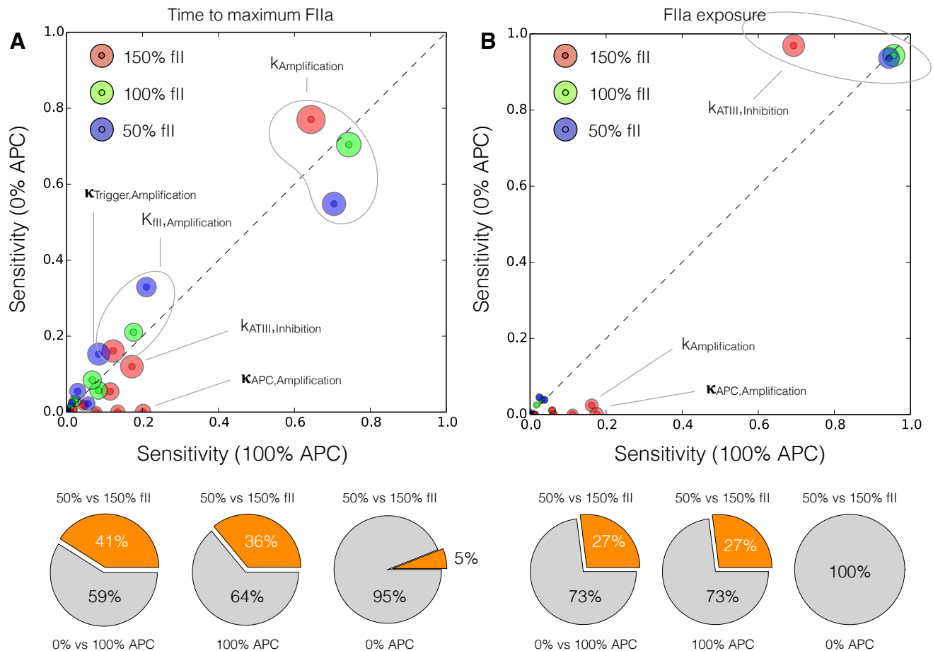
Figure 9. Global sensitivity analysis of the reduced order coagulation model with respect to the model parameters. (A) Sensitivity analysis of the thrombin peak time for different prothrombin levels (150%, 100% and 50% of the physiological value) as a function of activated protein C; (B) Sensitivity analysis of the thrombin exposure for different prothrombin levels (150%, 100% and 50% of the physiological value) as a function of activated protein C. Points denote the mean total sensitivity value, while the area around each point denotes the uncertainty in the sensitivity value. The gray dashed line denotes the 45° degree diagonal, if sensitivity values are equal for different conditions they will lie on the diagonal. Sensitivity values significantly above or below the diagonal indicate differentially important model parameters. The radius of the shaded region around each total sensitivity value was the maximum uncertainty in that value estimated by the Sobol method.
