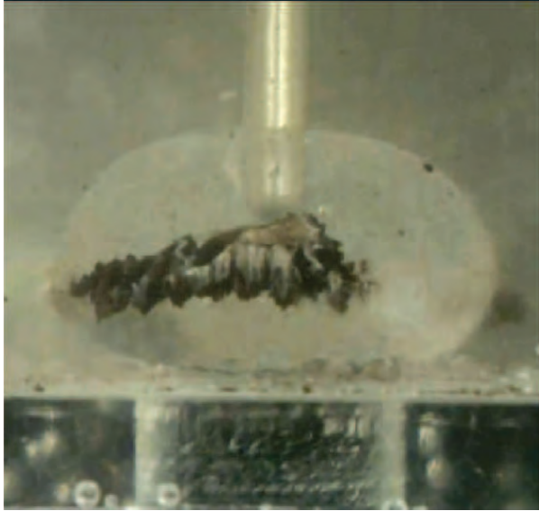
Figure 18. Indentation and large deformations of the porcine (2+years old) lens: (left) experiment, (right) simulation. The indenter has a 2mm diameter and a spherical tip and is lowered at 0.5mm/s until puncture of the capsule.
