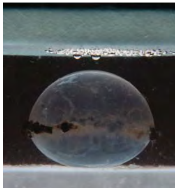
Figure 3.4: Shape of Lens (Anterior Surface Facing Down) Testing in Testing Platform, Showing Upper Load Platen.
