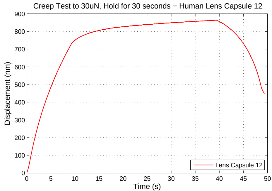
Figure 5.21: Graph of Nanoindentation Creep Test Human Lens Capsule 12 - Load to 30 \mu N, Hold for 30 seconds. The pre-load force necessary to get contact with the lens capsule is the cause of the non-zero starting force.
