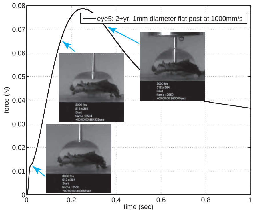
Figure 14. (top) Force versus time curve for a high strain rate puncture test on a 2+year old porcine lens. (bottom) Zoom in plot of the same curve, showing the peak load, and associated deformed lens images.
