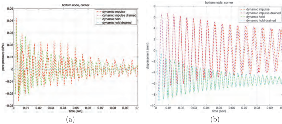
Figure 19: 50 Q27P8 element mesh results: (a) Plot of pore air pressure p_f versus time for the various analyses. (b) Plot of displacement d_y versus time for the various analyses.
