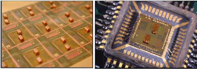
Figure 14: (left) Si oscillator circuit wafer with integrated high Q-factor out-of-plane coils and (right) oscillator chips after die singulation and packaging. (Original figure courtesy of Chris Chua, Xerox PARC.)
