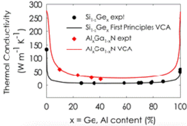
Figure 10: Thermal conductivity of SiGe and AlGa N alloys as functions of Ge and Al content. The plot shows experimental data as well as predictions of the Virtual Crystal Model (VCA) which shows the strong dependence on alloy composition. (Original figure and calculations courtesy of Sam Graham, Georgia Institute of Technology.)
