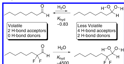
Scheme 1. Aldehyde Hydration Equilibria and H-Bonding Capability
