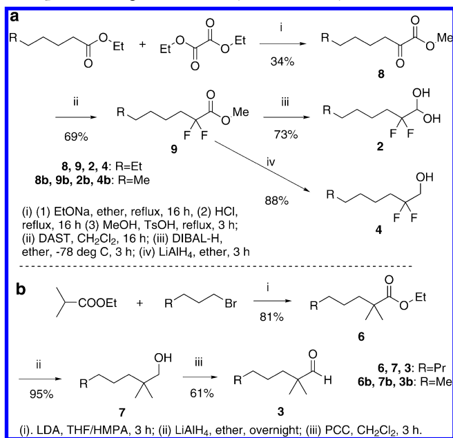
Scheme 2. Synthetic Routes to Compounds Used in Odorant Receptor Testing and NMR Hydration Study
