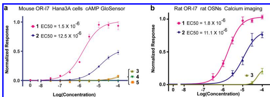
Figure 3. Dose–response curves for compounds 1–5 and rodent OR-I7. (a) Hana3A cells expressing mouse OR-I7 were exposed to odorants while cAMP production was monitored over a 30 min period. The summed response between 3 and 7.5 min is shown versus odorant concentration. (b) Rat olfactory sensory neurons infected with adenovirus expressing rat OR-I7 were assayed using calcium imaging during exposure to odorants 1–3.
