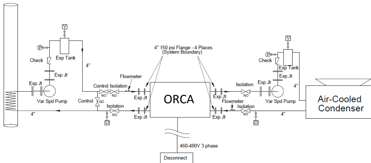
Figure 13. Installation Schematic
