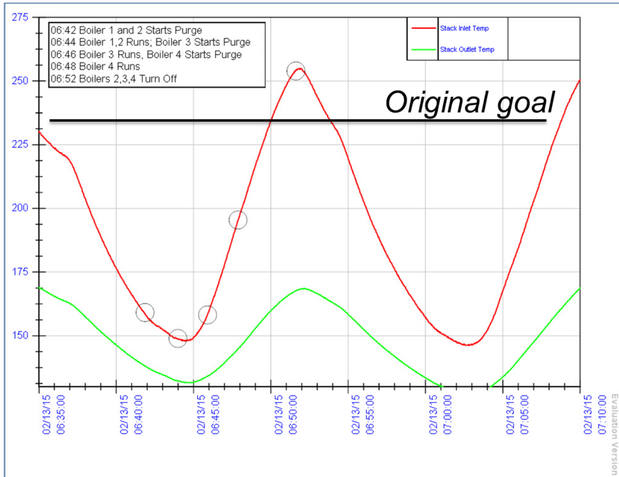
Figure 14. Heat Flows and Run Cycle of Boilers
