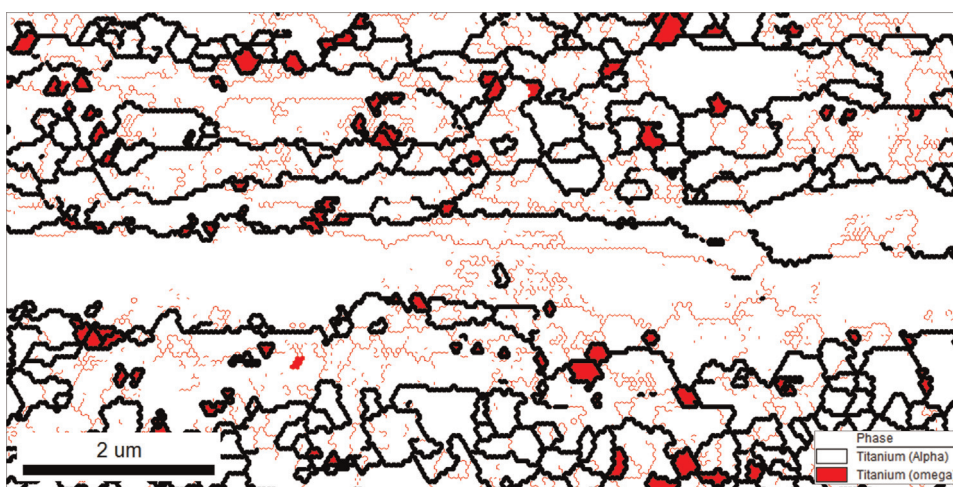
Fig. 2. Selected portion of an EBSD map for the alpha (white) and omega (red) phases taken from the longitudinal cross section of severely-deformed rod. In the map, LABs and HABs are depicted as red and black lines, respectively. (For interpretation of the references to color in this figure legend, the reader is referred to the web version of this article.).
