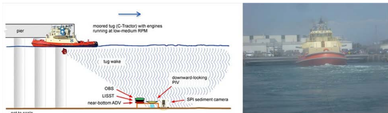
Figure 6-1. Field Study of Tugboat Propeller Wash at Pier 4-5 of Navy Base San Diego (Configuration of Instruments in Propeller Plume, Left, and Tugboat Tractor C-14 in Operation, Right).
