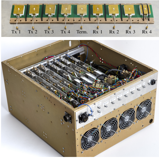
Fig. 2. ALSTAR prototype consists of a linear patch array with 4 transmitting and 4 receiving elements, and an 8-channel digital transceiver chassis.
