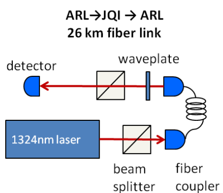
Fig. 58 Polarization stability experimental layout
