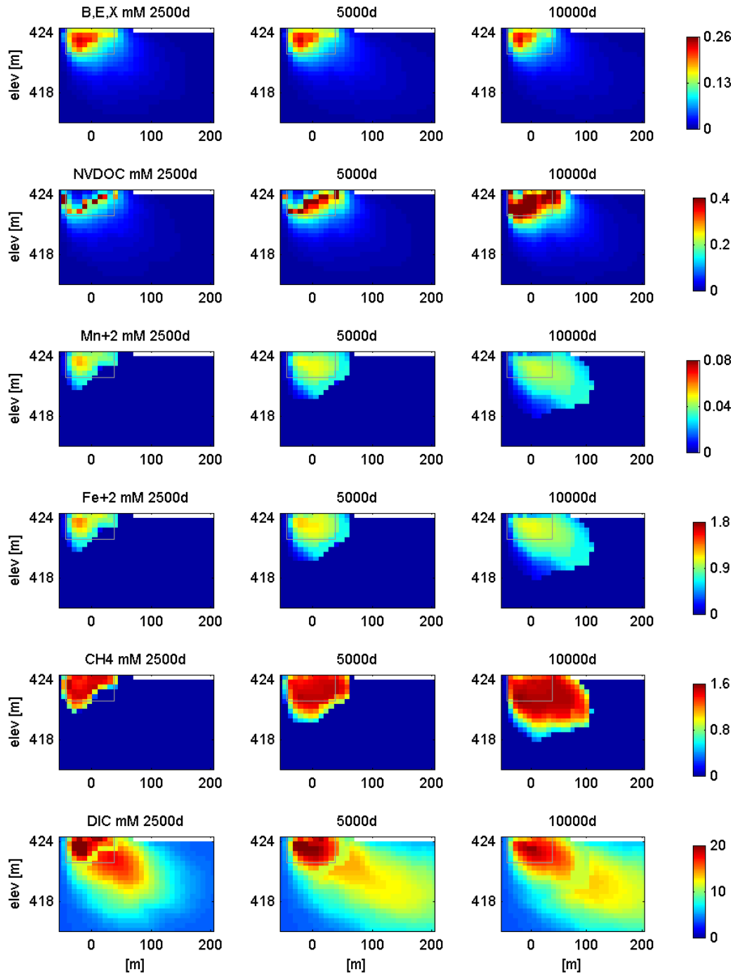
Figure 2.3. Model simulation results for six major redox species at three times corresponding to the observational time periods chosen for the data compilation.
