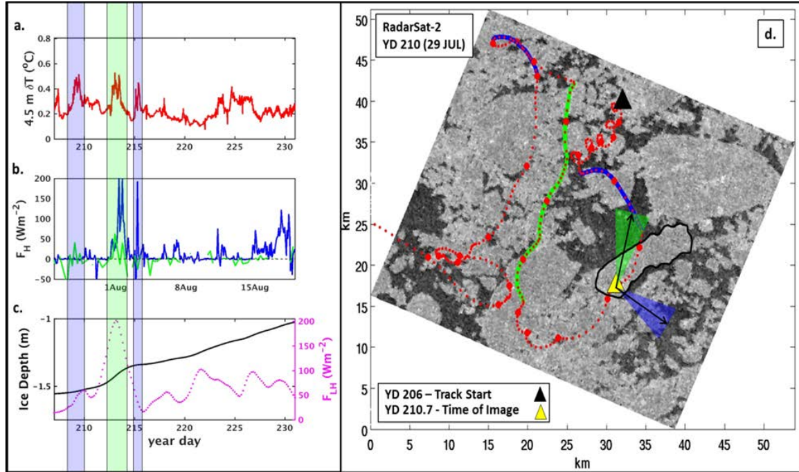
(a) 4.5 m \delta T , (b) 4.5 m (blue) and 6.5 m (green) turbulent heat fluxes, (c) 3-day averaged sea ice bottom interface depth (black) and latent heat fluxes (magenta dots), and (d) RadarSat-2 image (YD 210.7) overlaid with MIZ C2 GPS track (red dots) between YD 206 (black triangle, start time of time series plots in Figs. 2.13a, 2.13b, and 2.13c) and YD 216. The time periods of interest are color coded in blue and green along the GPS track and on the corresponding supporting plots (a, b, c). To determine the direction of ice motion during the different time periods, color coded vector triangles with direction arrows are plotted over the location of C2 at the time the image was acquired (yellow triangle).
