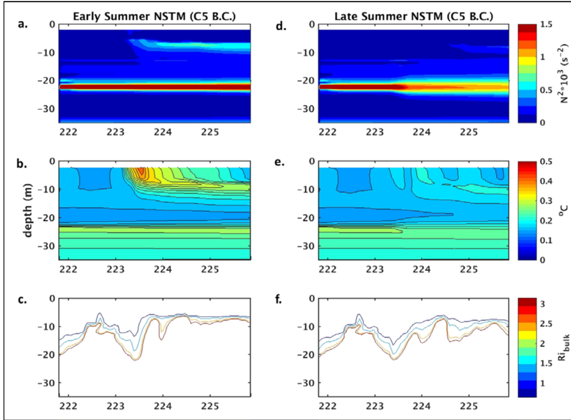
LTC model output of the (a) N^2 and (b) temperature above freezing, and (c) contours of Ri_{bulk} (0.65, 1.3, 1.95, 2.6) for the early summer case using MIZ C5 air-ice-ocean conditions. For this case, 0.25 m of freshwater was added to the model on YD 223. (d-f) Same format as the left-hand panels but for the late summer case using observed freshwater input (0.1 m) during the MIZ-KOPRI Ice Camp.
