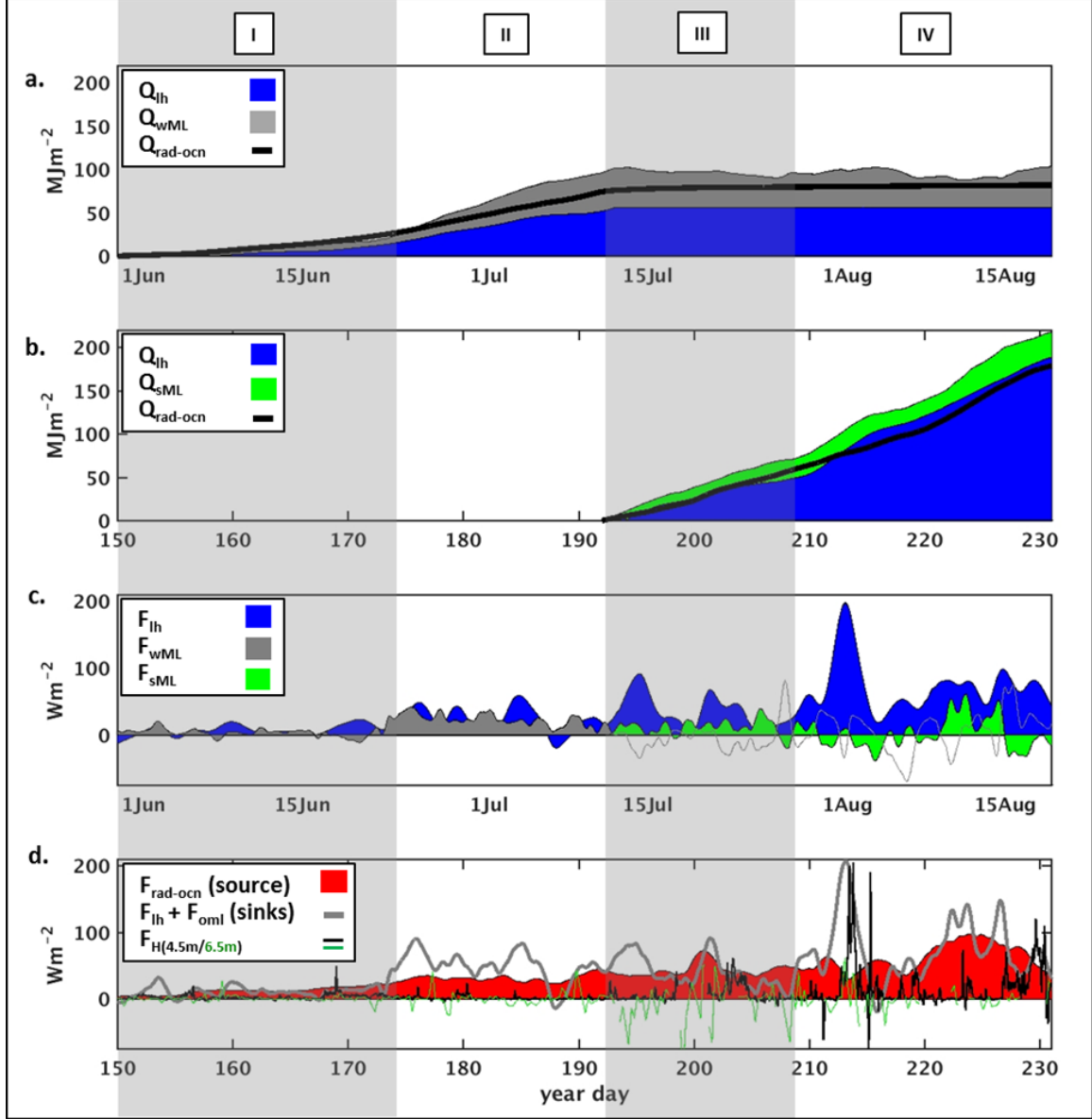
1-D Heat Budget Overview at MIZ C2 to estimate the magnitude of ocean absorbed solar radiation (source) and how it is redistributed between latent heat losses (sink #1) and heat storage (sink #2). (a) Winter mixed layer heat budget: 3-day averaged time series of shortwave source term Q_{rad-ocn} (black line), wML heat storage sink term Q_{wML} (gray), and latent heat sink term Q_{lh} (blue). (b) Summer mixed layer heat budget: 3-day averaged time series of shortwave source term Q_{rad-ocn} (black line), sML heat storage sink term Q_{sML} (green), and latent heat sink term Q_{lh} (blue). (c) The 3-day averaged latent heat flux term F_{lh} (blue) and OML heat storage flux terms F_{wML} (gray) and F_{sML} (green), and (d) the 3-day averaged ocean radiative flux term F_{rad-ocn} (red), sum of latent heat and OML heat storage flux terms F_{lh} + F_{oml} (gray line), and turbulent heat fluxes at 4.5 m and 6.5 m ( F_{H(4.5m/6.5m)} , black and green lines, respectively).
