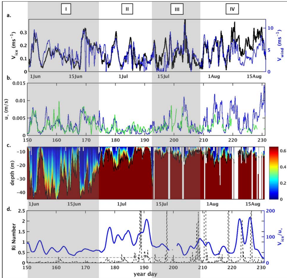
(a) 2 m winds (blue) and ice speeds (black), (b) 4.5 m (blue) and 6.5 m (green) turbulent friction velocities, (c) bulk Richardson number ( Ri_{\text{bulk}} ) showing estimated turbulent penetration ( Ri_c = 0.65 ), and (d) the ratio of ice speed to 4.5 m friction velocity ( V_{\text{ice}}/u_{*(4.5\text{ m})} ) (blue) and the 5.5 m Richardson number ( Ri ) (black).
