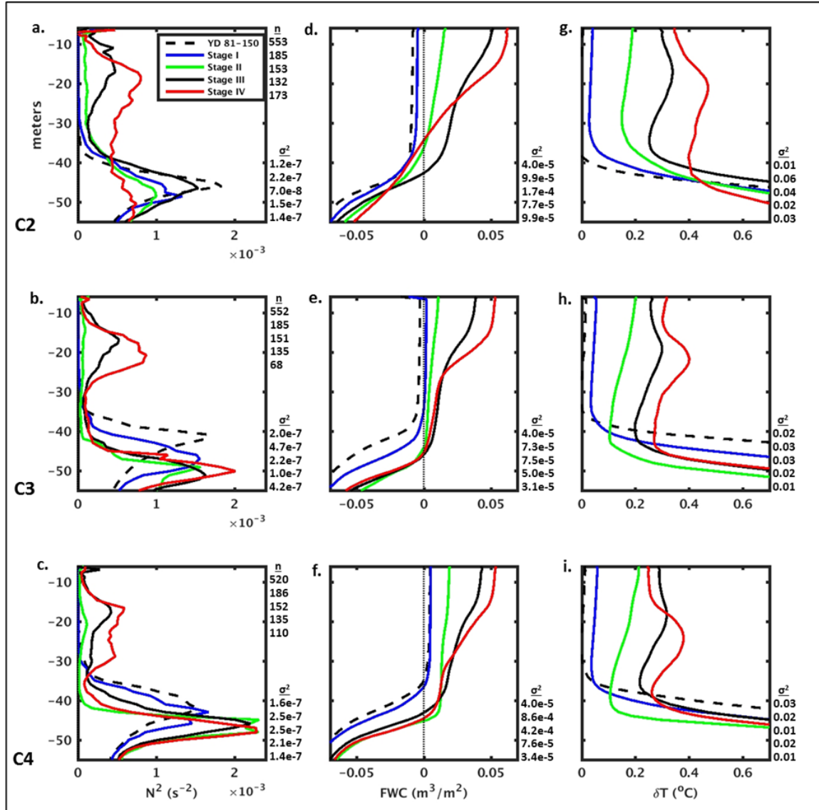
Upper ocean profiles of stage-averaged (a, b, c) N^2 , (d, e, f) freshwater storage (FWC), and (g, h, i) \delta T for clusters 2-4 (see legend). Rows correspond to observations from C2, C3, and C4, respectively. Number of profiles ( n ) and the mean variance statistics ( \sigma^2 ) across all depths for each stage are provided on the right side of the plot.
