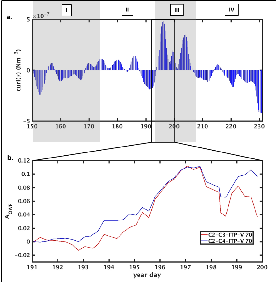
a) 2-day averaged wind stress curl ( \text{curl}(\tau) ) estimated from MIZ C2-C4 and ITP-V 70 observations in the Canada Basin. (b) Estimation of open water fraction ( A_{\text{OWF}} ) from divergence between the MIZ sensors using the triangle area differencing method (Stanton et al. 2012). Triangle area differencing was calculated on C2, C3, and ITP-V 70 (red) and C2, C4, and ITP-V 70 (blue) every 6 h.
