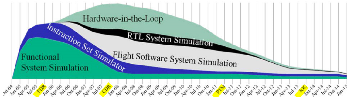
Figure 14. Simulation Fidelity of the MK6LE Across the Development Cycle.
