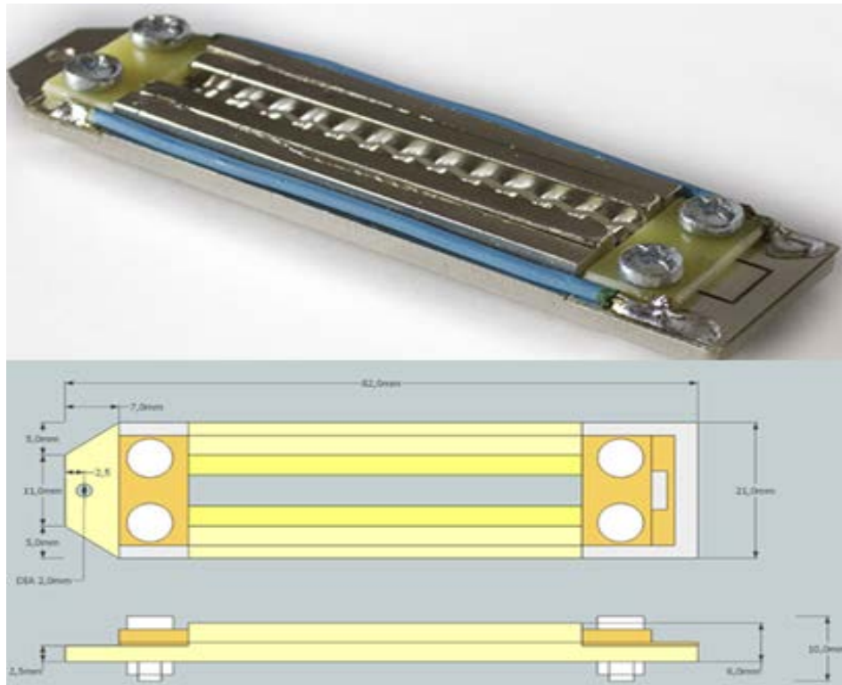
Figure 17. True Ribbon Transducer. Source [8].
