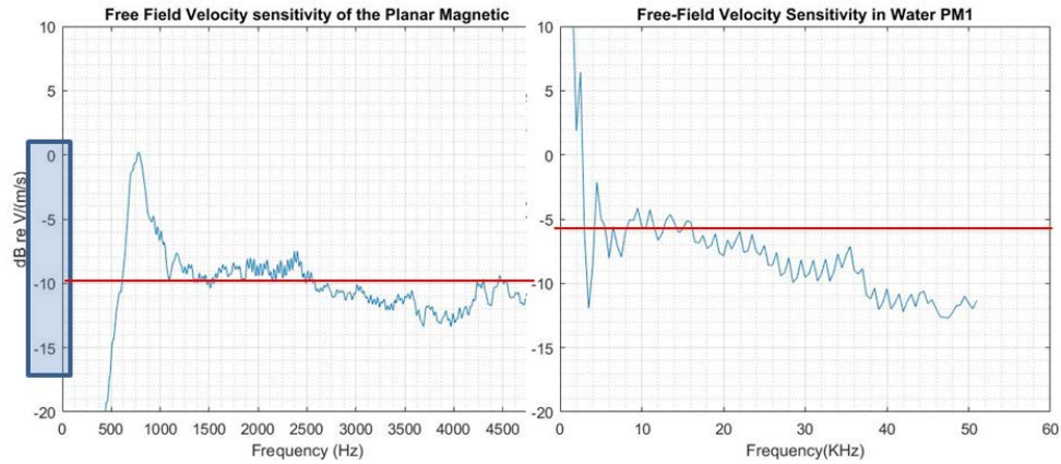
Figure 97. Comparison of Both Velocity Sensivities in Air and Water.
