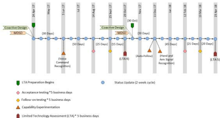
Figure 4. LTA Timeline
