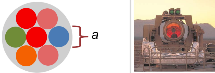
Figure 3.1.4: Beamlets bundled side by side at the beam director aperture is shown on the left and the actual beam director is shown on the right.
