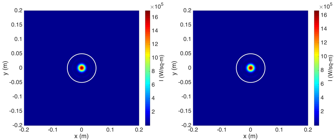
Figure 6.1.9: For the 13 coherent beamlets case with 1kW output power, the target irradiance patterns for the propagation model (left) and WaveTrain (right).
