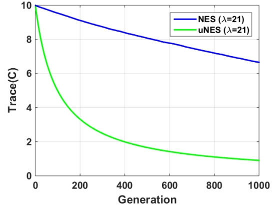
(b) Trace of C Progression on a 10-D Parabola
