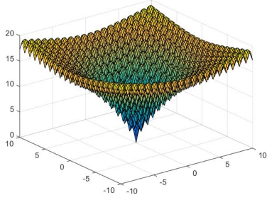
(a) Ackley
