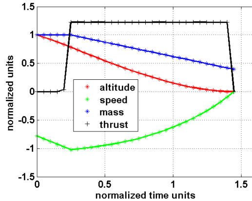
Figure C.1. Unscented RCGA 30-node lunar lander trajectory
