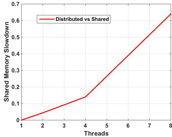
Figure 2.17. Shared memory coherency penalty curve
