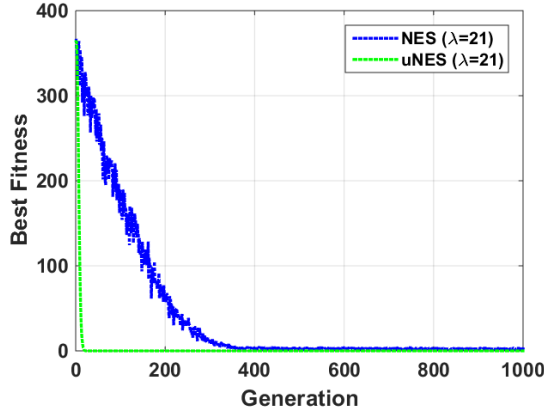
(a) Fitness progression on a 10-D Parabola
