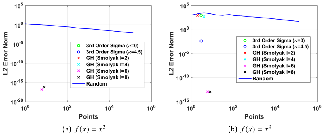
Figure 7.1. Accuracy of \nabla_{\mu} J(\mu, \sigma) on the 1-D functions f(x) = x^2 and f(x) = x^9 ( \mu = 0 , \sigma = 1 )
