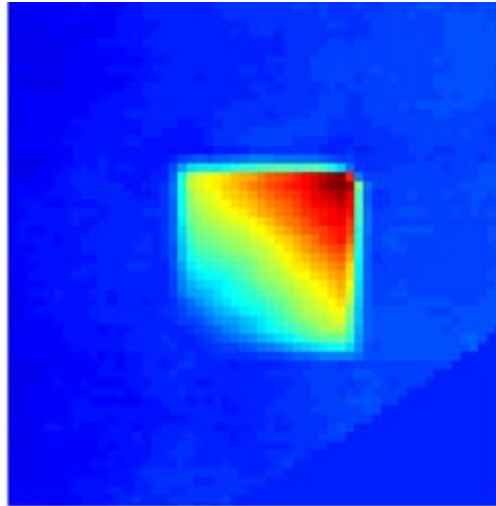
Boston 492-DM single actuator deflection with 100V applied. The surface colors represent the relative height of a pixel in relation to one another. Dark red is a high spot while blue indicates a lower value. The image shows that the segmented surface appears to be slanted which is a result of nonlinearities in the system. Since the surrounding area around the segment is blue, a low spot, this indicates that the segment is being poked.
