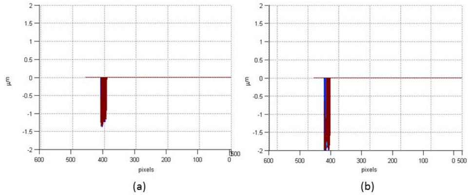
Variance in actuator piston height for actuator 8 (a) and actuator 58 (b) given the same 100 volts. An approximate 0.8 \mu m difference exists between these actuators despite the same identical voltages.
