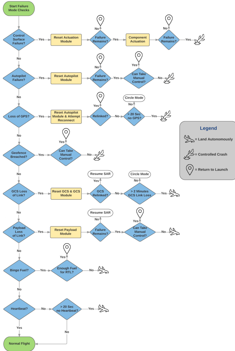
Figure 35. Failure Mode and Failsafe Behavior Order of Operations
