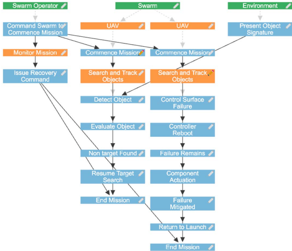
Figure 23. MP Sequence Diagram – Control Surface Failure (Scope = 2)
