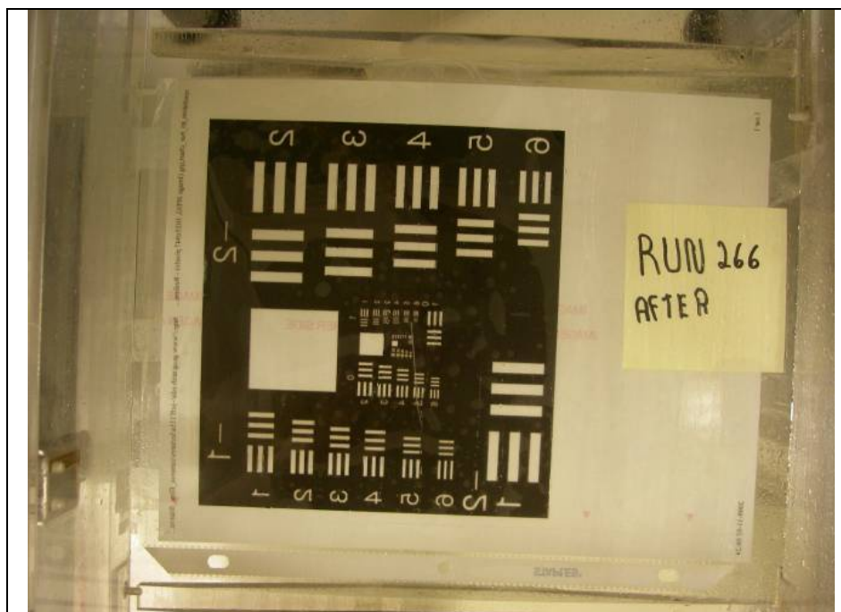
EcoFlo @ -20°C, NominalH 2 O Reduction, 4mm Initial Fluid Thickness, After 15 min Run Time (Run #266)
