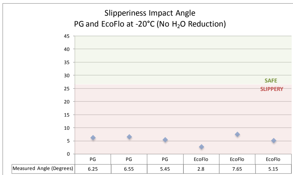
Slip Measurements at -20°C, with No H 2 O Reduction Prior to Test
