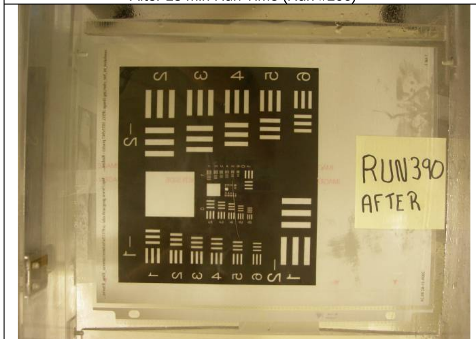
EcoFlo @ -20°C, NominalH 2 O Reduction, 4mm Initial Fluid Thickness, After 15 min Run Time (Run #390)
