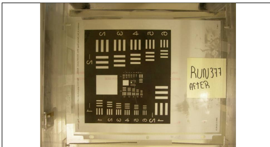
OCTAFLO EF @ 0°C, 0% H_2O Reduction, 1mm Initial Fluid Thickness, After 5 min Run Time (Run #377)
