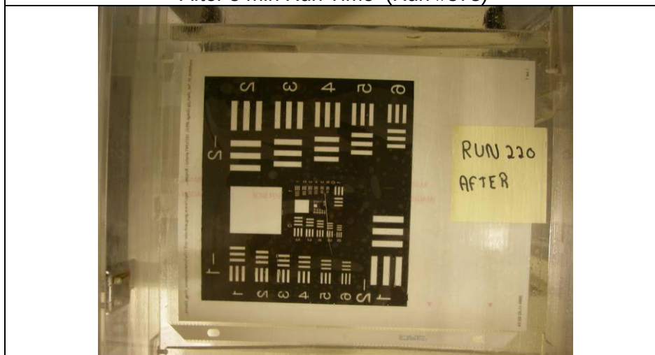
EcoFlo @ 0°C, 0% H_2O Reduction, 4mm Initial Fluid Thickness, After 5 min Run Time (Run #220)
