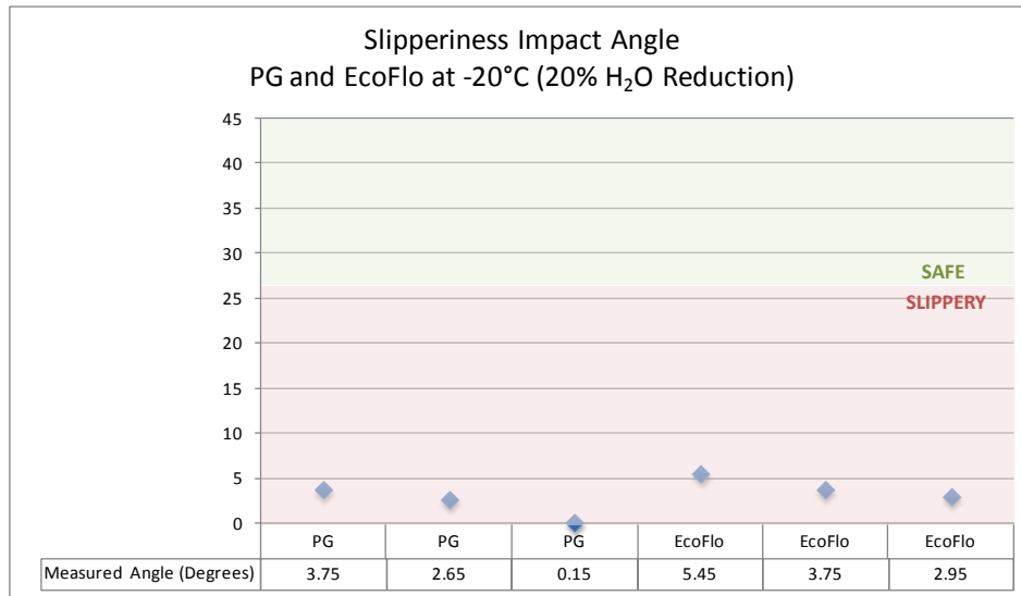
Slip Measurements at -20°C, with 20% H 2 O Reduction Prior to Test
