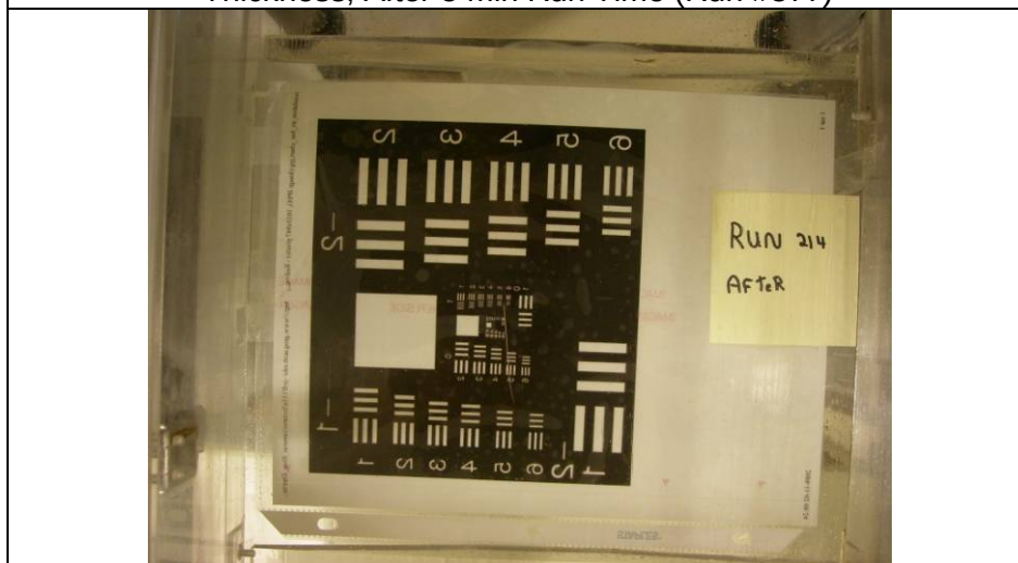
EcoFlo @ 0°C, 0% H_2O Reduction, 1mm Initial Fluid Thickness, After 5 min Run Time (Run #214)
