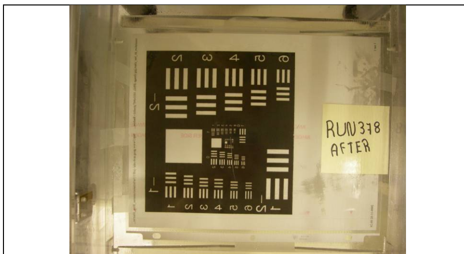
OCTAFLO EF @ 0°C, 0% H_2O Reduction, 4mm Initial Fluid Thickness, After 5 min Run Time (Run #378)
