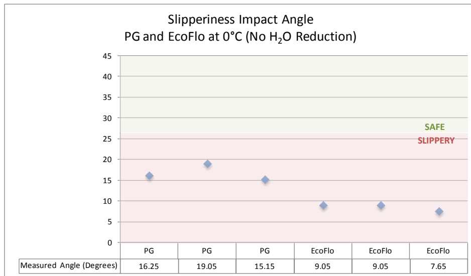
Slip Measurements at 0°C, with No H 2 O Reduction Prior to Test
