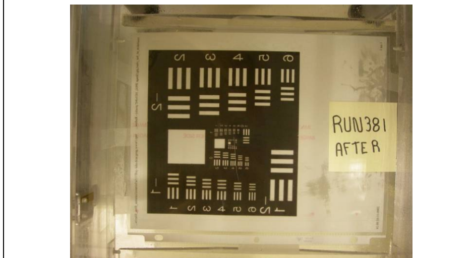
EcoFlo @ 0°C, 0% H_2O Reduction, 1mm Initial Fluid Thickness, After 10 min Run Time (Run #381)
