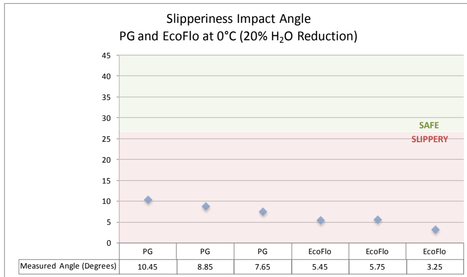
Slip Measurements at 0°C, with 20% H 2 O Reduction Prior to Test
