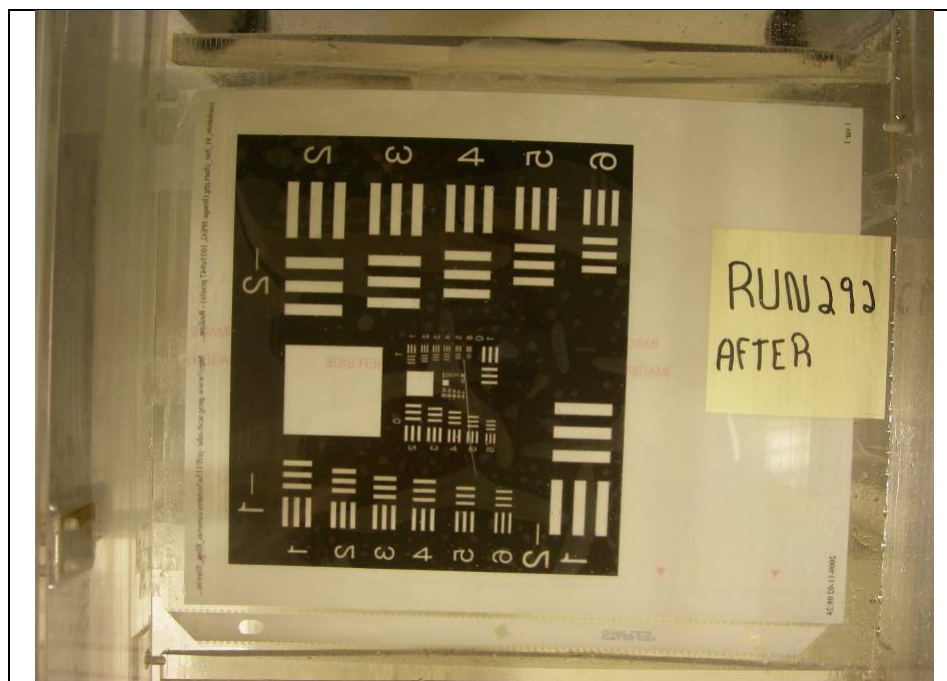
EcoFlo @ 0°C, 40% H_2O Reduction, 1mm Initial Fluid Thickness, After 5 min Run Time (Run #292)
