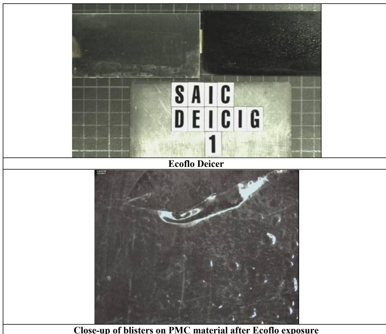
Figure 3. Photos of Sandwich Corrosion Samples
