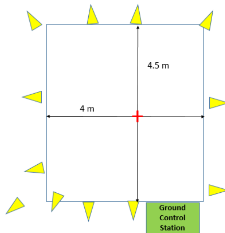
Figure 6. ASEIL Layout
