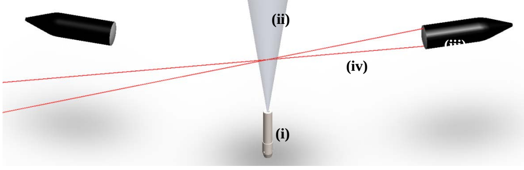
Fig. 17-Simplified diagram of the phase Doppler interferometer with the spray nozzle (i), plume (ii), laser transmitter (iii), laser beams (iv), and receiver (v).
