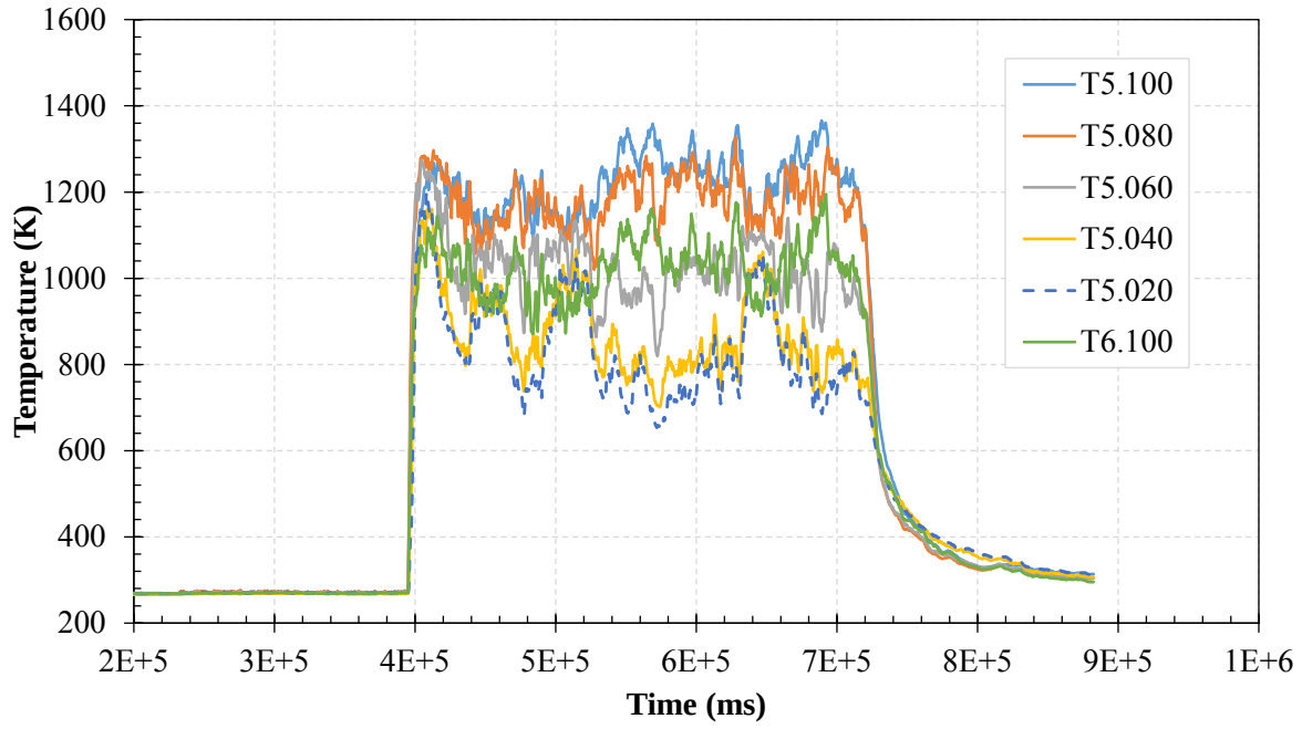
Fig. 48-Time-history plot of stage 3 thermocouples.
