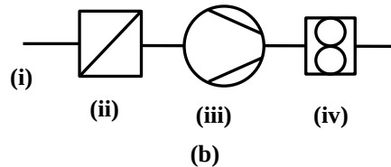
Fig. 8-(a) Instrumentation rake for extracting plume samples and measuring plume temperature and (b) plumbing diagram. The rake inlet (i), filter (ii), vacuum pump (iii), and displacement meter (iv).
