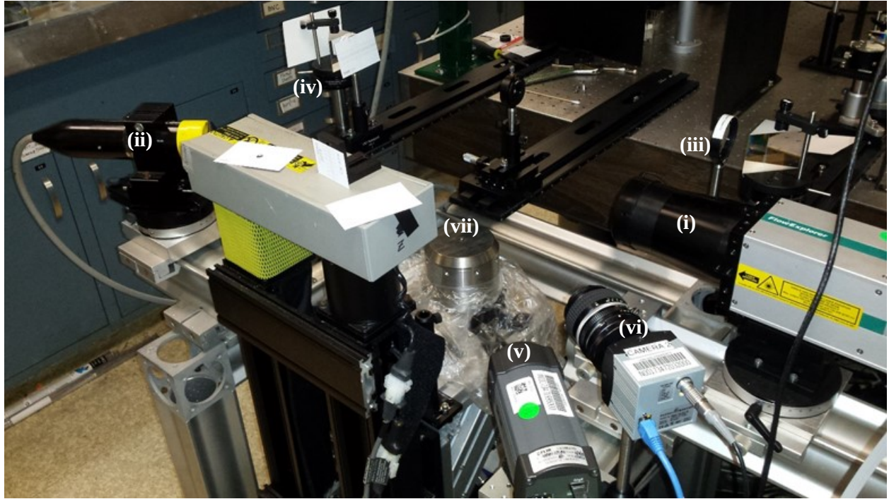
Fig. 21-Photograph of the instrumentation layout that surrounded the laboratory spray burner. These include the PDA transmitter (i), PDA receiver (ii), CARS transmission optics (iii), CARS receiving optics (iv), IR camera (v), high-speed visible camera (vi), and spray burner (vii).
