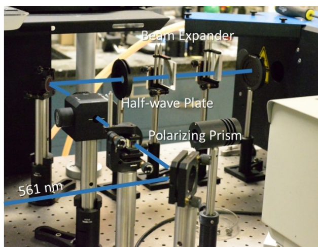
Fig. 33-Image of the beam expander, half-wave plate and polarizing prism through which the 561 nm beam passes.
