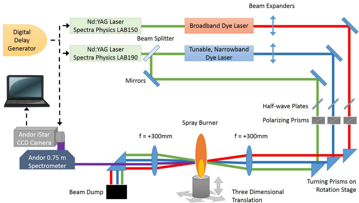
Fig. 26-Schematic diagram of the DPCARS and spray burner system.
