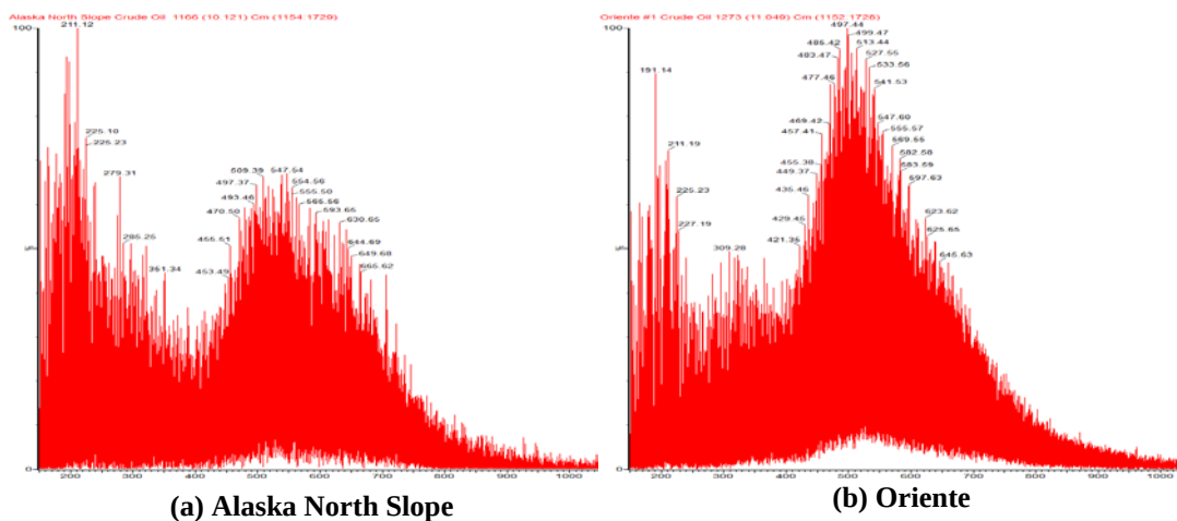
Fig. 67-Comparative ASAP mass spectra of Alaska North Slope and Oriente Crude Oil averaged between 10 and 15 min.
