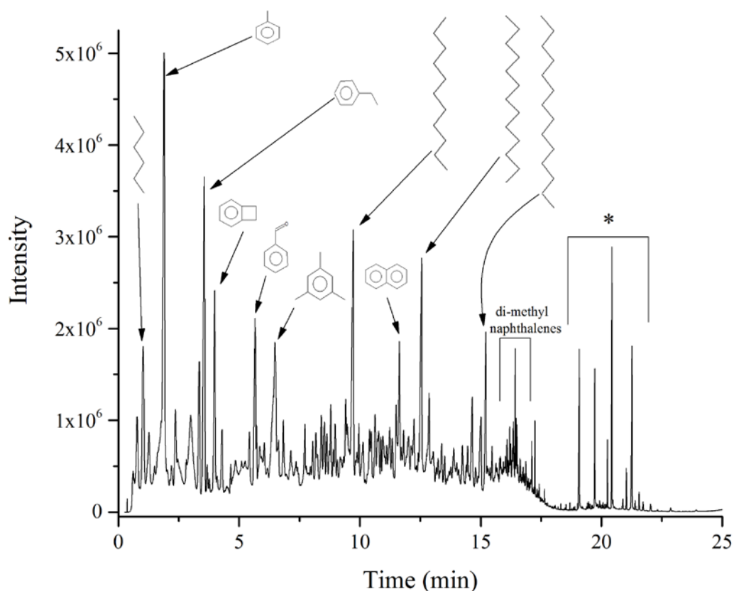
Fig. 79- Spectra from exhaust samples gathered in a sorbent tube for 25% emulsified ANS burned in a laboratory spray plume with \dot{m}_{\text{Air}} = 2.9 \times 10^{-4} kg/s, \dot{V}_{\text{Oil}} = 23.2 mL/min (see Table 3). * denotes major peaks identified in Fig. 78 from the baseline neat ANS crude
