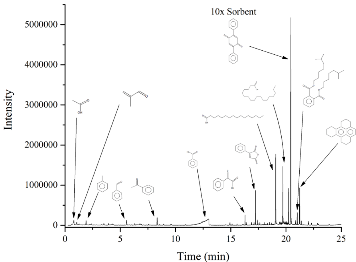
Fig. 78-Baseline spectra from exhaust samples gathered in a sorbent tube for neat ANS burned in a laboratory spray plume with \dot{m}_{\text{Air}} = 2.9 \times 10^{-4} \text{ kg/s} , \dot{V}_{\text{Oil}} = 23.2 \text{ mL/min} (see Table 3).
