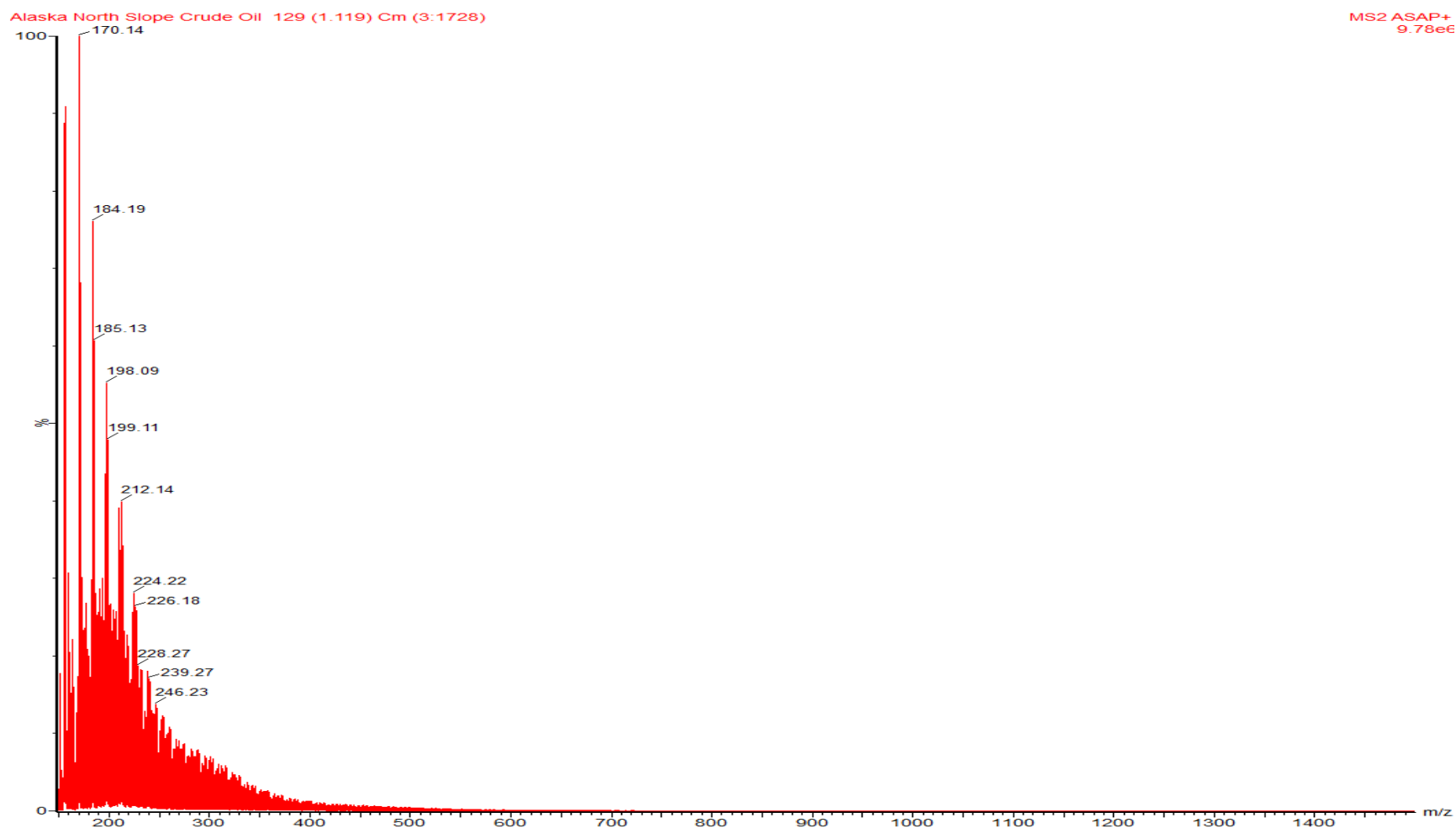
Fig. 65-ASAP mass spectra of Alaska North Slope Crude Oil averaged over 15 min.
