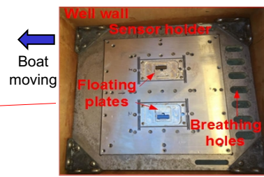
Shear sensor
