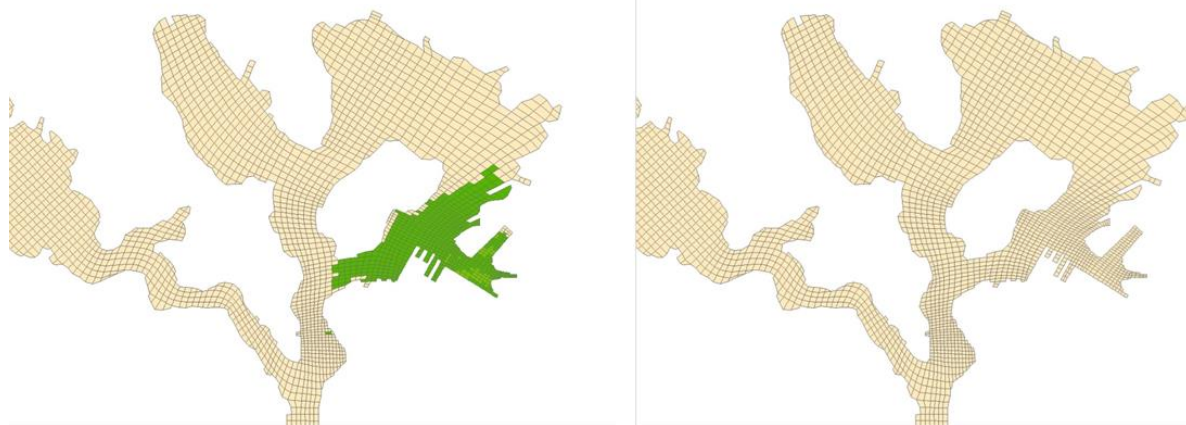
Figure 6-93. Simulated silt-particle-bound copper concentrations at bottom layer at t = 30 hours (left), and t = 120 hours (right) after prop-wash resuspension.
