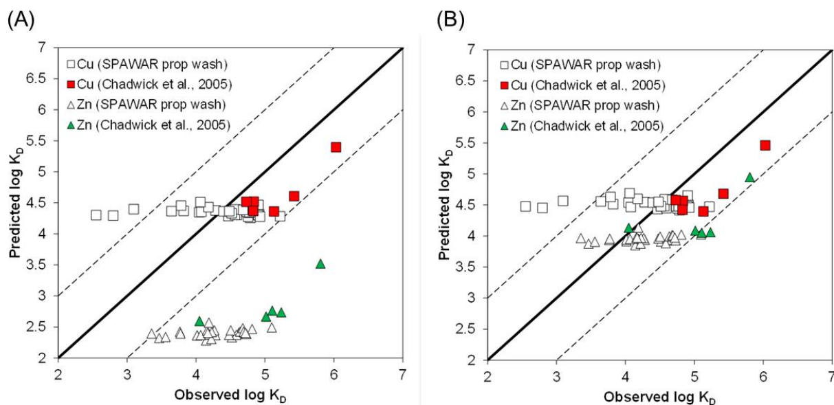
Figure 6-40. Performance assessment plot for copper (Cu, squares) and zinc (Zn, triangles) for the Chadwick et al. (2005) dataset (filled symbols) and the SPAWAR prop wash dataset (hollow symbols). The analysis was made using (A) default model parameters, and (B) with hardness cation (calcium and magnesium) binding to DOC, POC, HFO, and HMO turned off.
