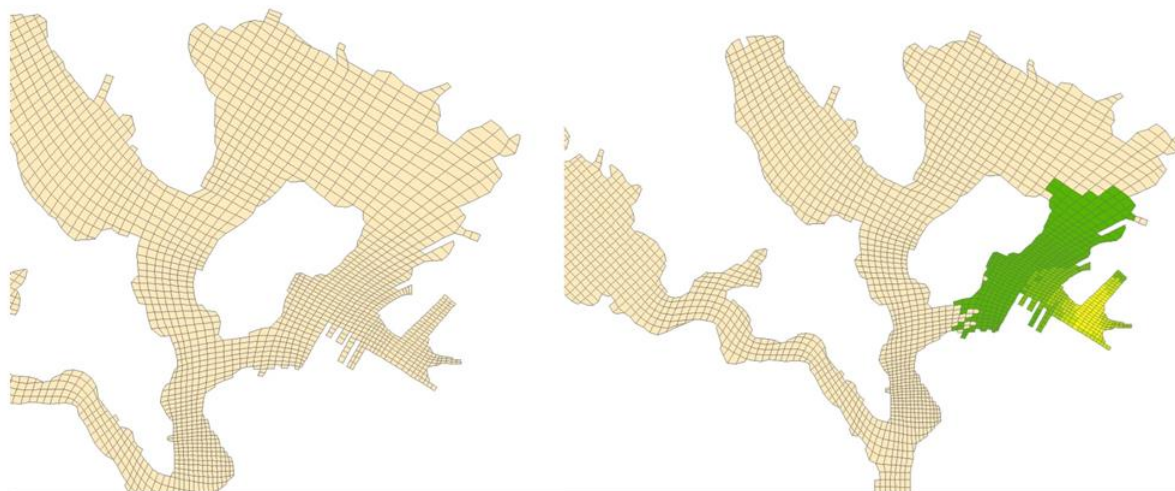
Figure 6-92. Simulated silt-particle-bound copper concentrations at surface (left), and bottom layer (right) 18 hours after prop-wash resuspension.
