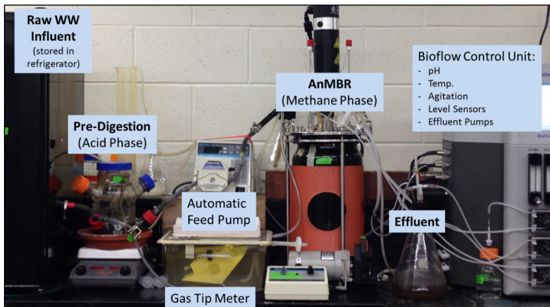
Figure 6. Continuous AnMBR system physical setup.
