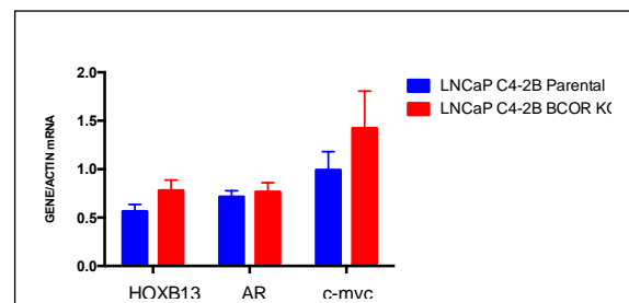
Fig 5. Ablation of BCOR does impact AR or HOXB13 levels. LNCaP C4-2B cells were transfected with BCOR CRISPR/Cas9 gene editing constructs. Relative quantitation of HOXB13, AR and c-myc mRNA levels in were examined. Actin is used as a normalization control. Error bars denote 95% confidence intervals.
