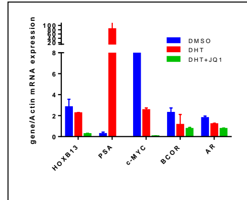
Fig 1. Analysis of AR, BCOR and HOXB13 mRNA expression in androgen stimulated and BET inhibitor treated PC cells.
