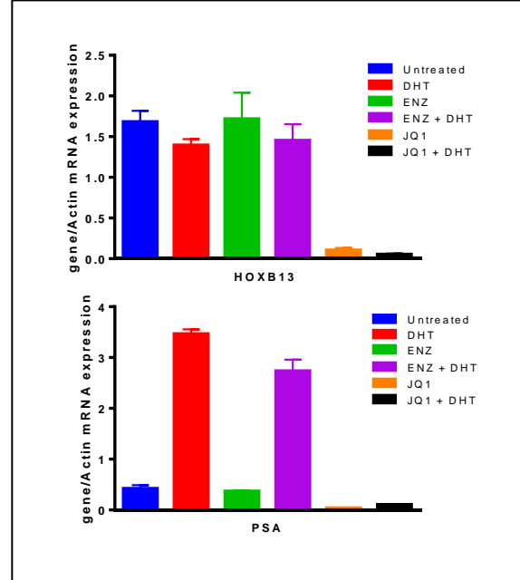
Fig 4. HOXB13 mRNA expression is androgen independent, resistant to enzalutamide but affected by BRD4 inhibitor, JQ1. Relative quantitation of HOXB13 and PSA mRNA levels in LNCaP cells treated with JQ1 or Enzalutamide (16h). Actin is used as a normalization control. Error bars denote 95% confidence intervals.
