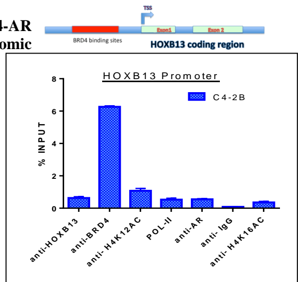
Fig 7. HOXB13 is epigenetically regulated by the BET bromodomain protein BRD4 in CRPC. A-B. Schematic of HOXB13 genomic region indicating the potential BRD4 binding sites. TSS- Transcription Start Site. CHIP-qPCR was performed with extracts prepared from the metastatic PC cell line C4-2B with various antibodies (anti-BRD4, anti-H4K12Ac, anti-AR, anti-H4K16Ac and IgG) and analyzed for HOXB13 promoter and enhancer region. Set 14 primer is 1kb from TSS.
